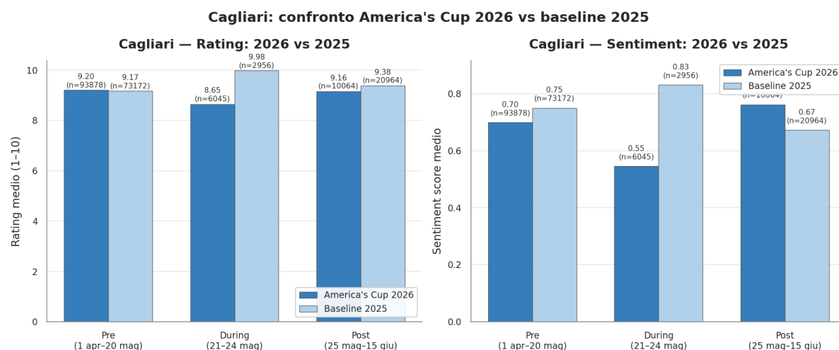
Figure 15: Confronto Cagliari 2026 vs 2025
