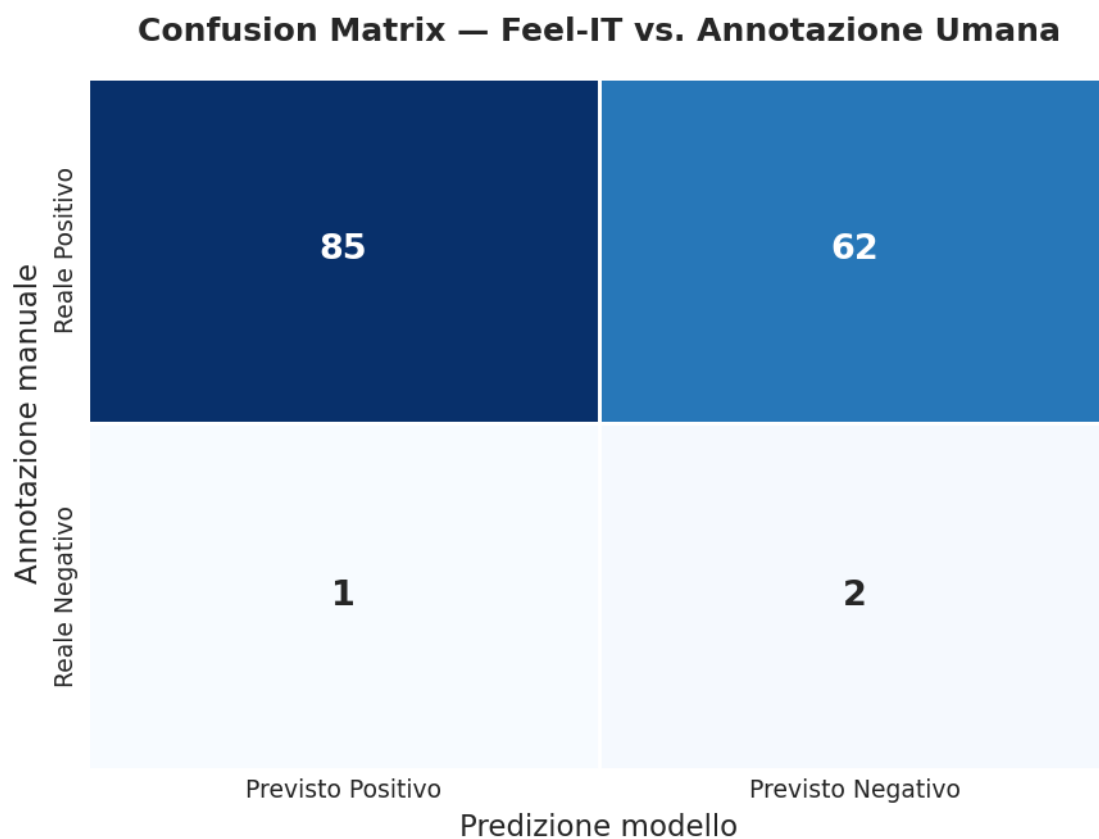
Figure 16: Confusion matrix Feel-IT
