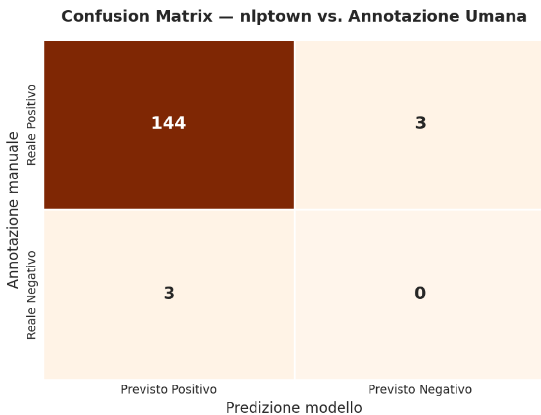
Figure 18: Confusion matrix nlptown
