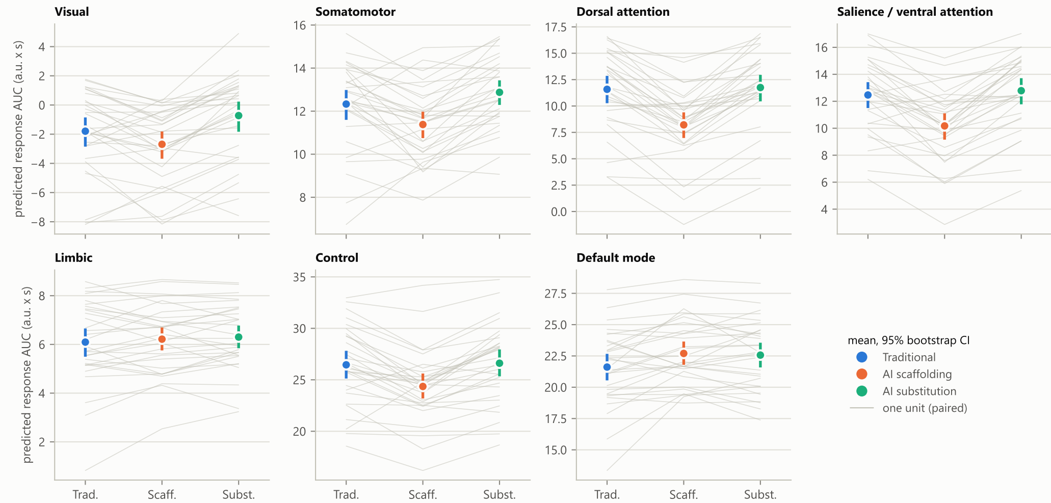
Figure 3. Predicted network-level responses by condition (TRIBE v2, 220 wpm, area-weighted AUC)
