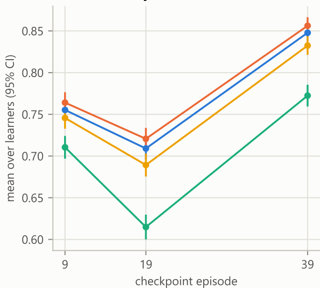
unaided accuracy
