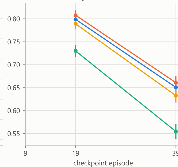
retention accuracy
