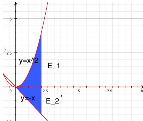
Figura 2.50: E = \{(x, y) \in \mathbb{R}^2; 0 \leq x \leq 2, -x \leq y \leq x^2\} .
