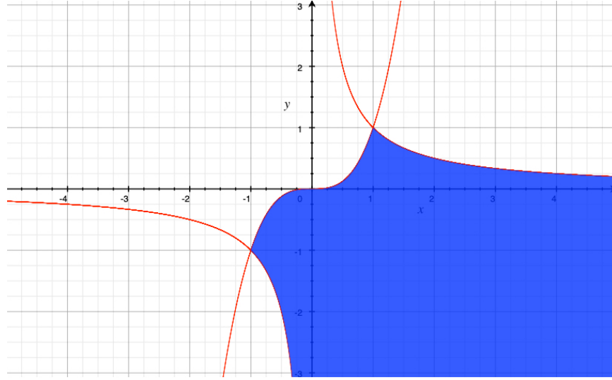
Figura 2.17: Grafico di E = \{(x, y) \in \mathbb{R}^2 \mid x^3 - y > 0, \sqrt{1 - xy} \neq 0, 1 - xy \geq 0\} = \{(x, y) \in \mathbb{R}^2 \mid y < x^3, 1 - xy > 0\} .
