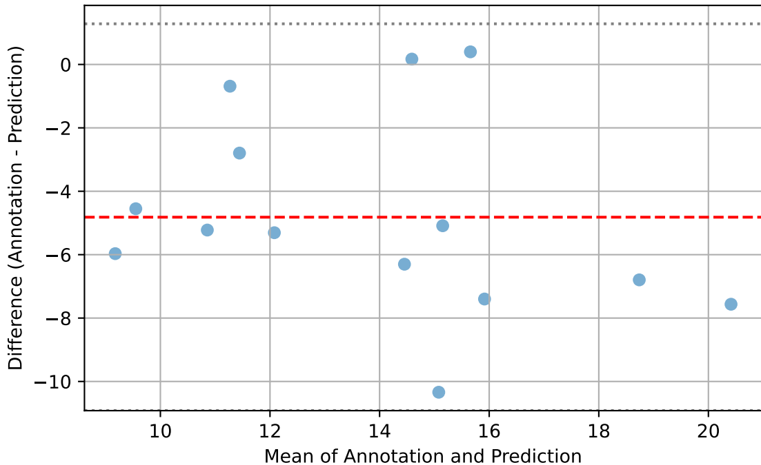
Bland-Altman Plot for tapsesep
