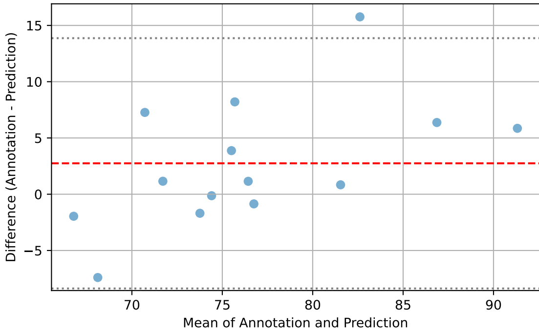
Bland-Altman Plot for rvldsep
