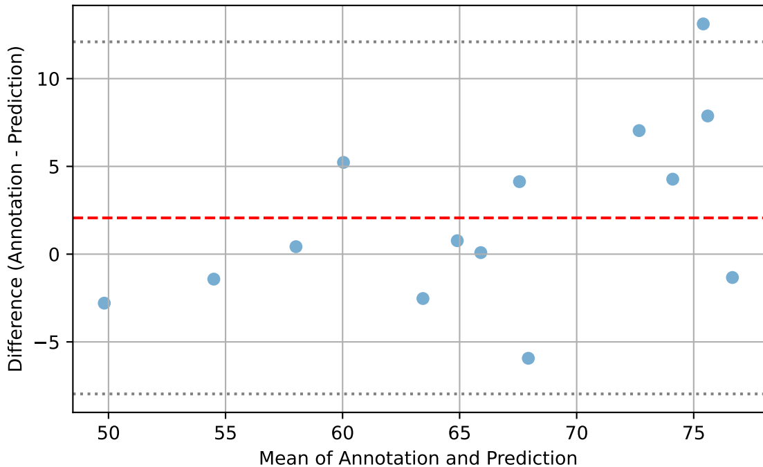
Bland-Altman Plot for rvlsfw
