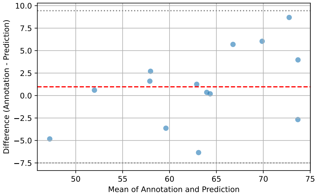
Bland-Altman Plot for rvlsmid
