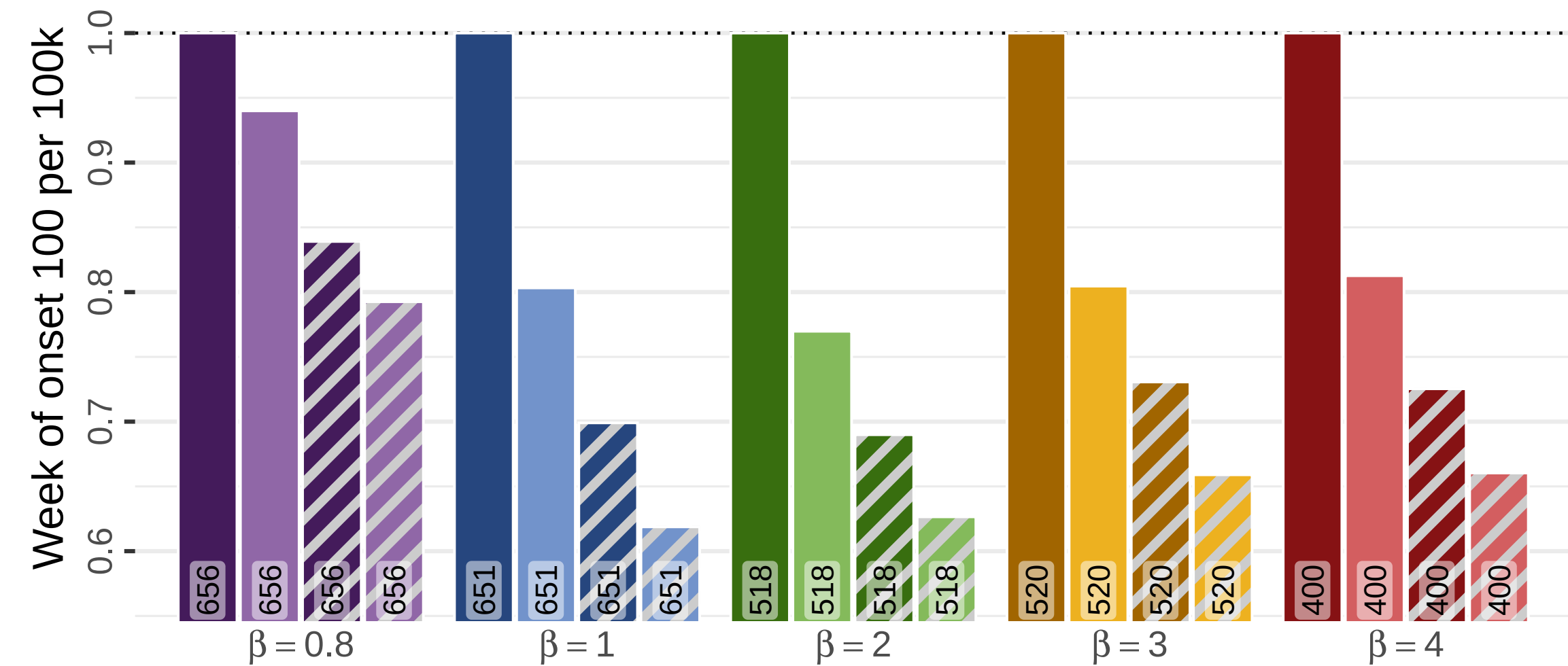
Mean MAE
