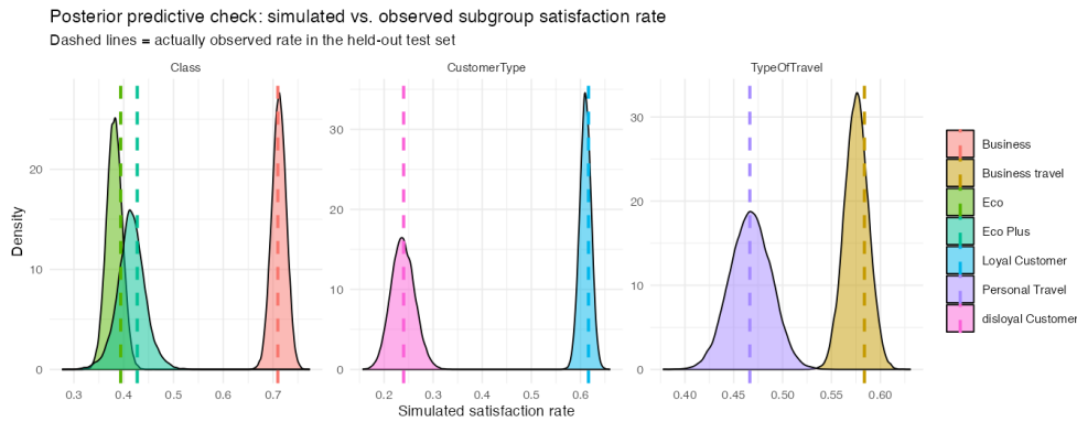
Figure 9. Posterior predictive check by subgroup. Densities are the simulated satisfaction rates; dashed lines mark the rates actually observed in the held-out set.
