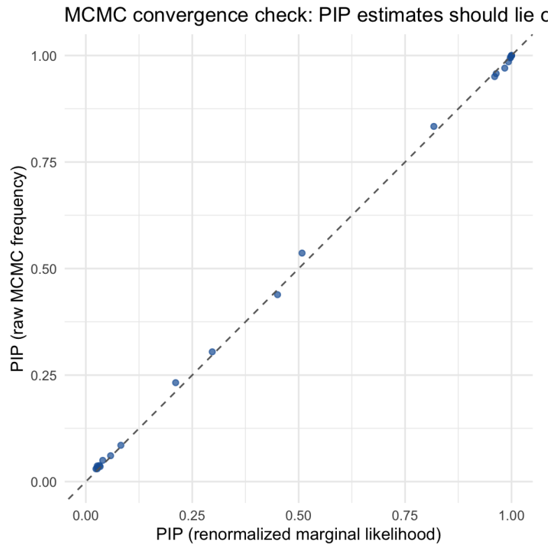
Figure 15. MCMC convergence check. Renormalised-marginal-likelihood inclusion probabilities (x-axis) against raw MCMC-frequency inclusion probabilities (y-axis); points lying on the dashed diagonal indicate the two estimates agree.
