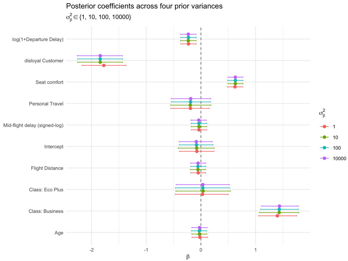
Figure 6. Posterior coefficients of the vague-prior logit model across four prior variances.
