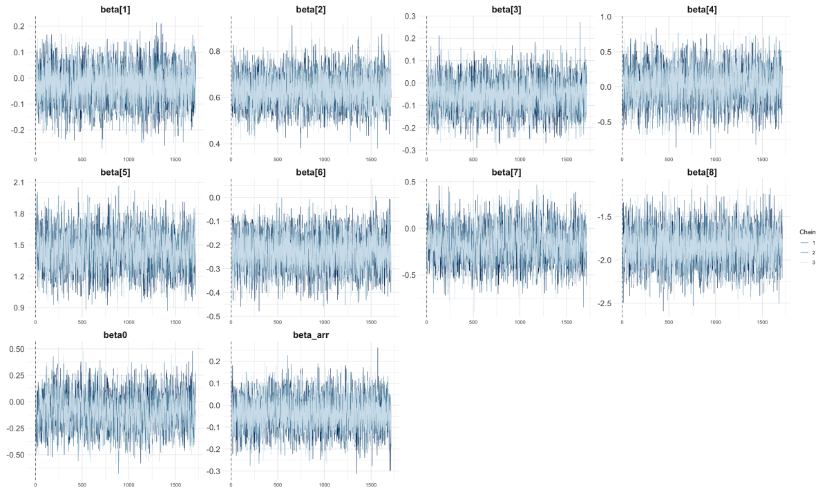
Figure 11. MCMC traceplot of the baseline logit model.
