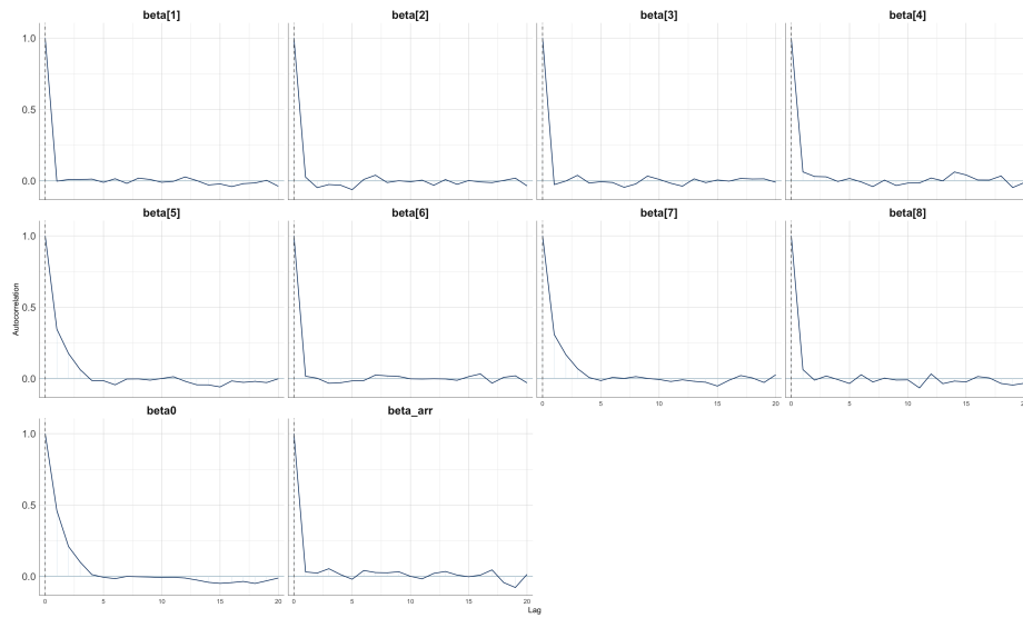
Figure 13. MCMC ACF plots of the baseline logit model (2nd chain).
