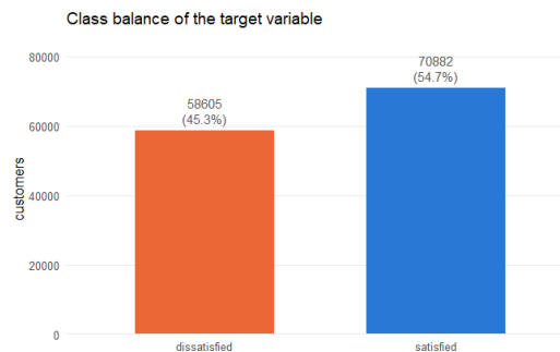
Figure 1. Target variable class balance
