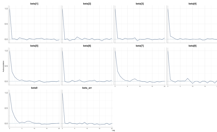
Figure 14. MCMC ACF plots of the baseline logit model (3rd chain).
