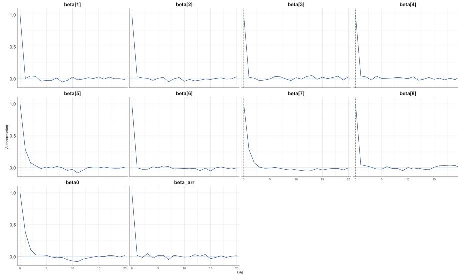
Figure 12. MCMC ACF plots of the baseline logit model (1st chain).
