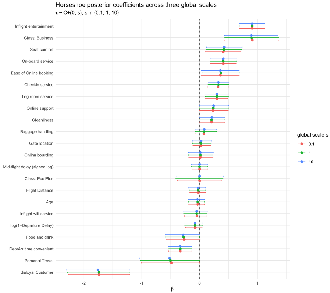
Figure 7. Horseshoe posterior coefficients across three global scales, ordered by shrinkage weight at the default scale.
