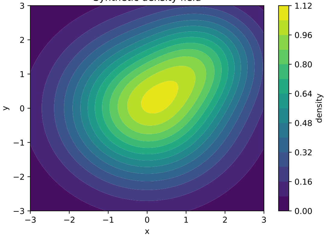
Synthetic density field
