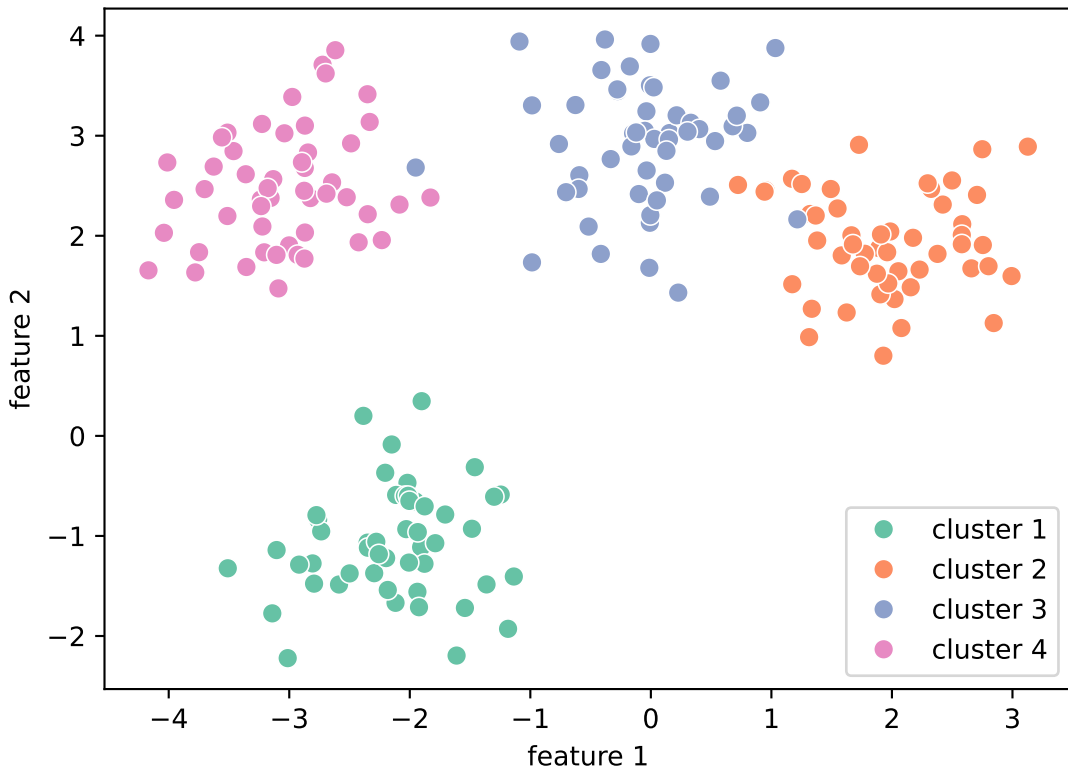
Cluster assignment
