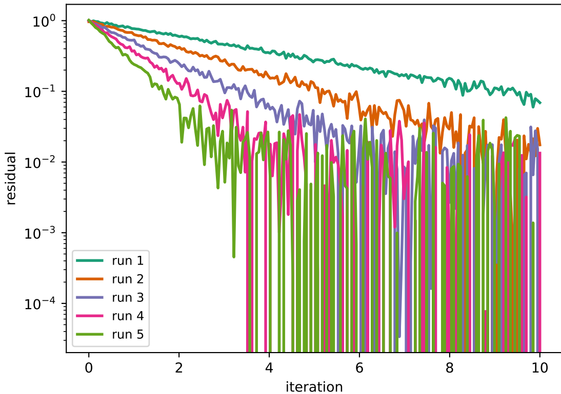
Convergence curves
