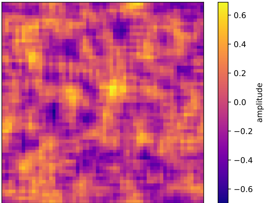
Smoothed noise field
