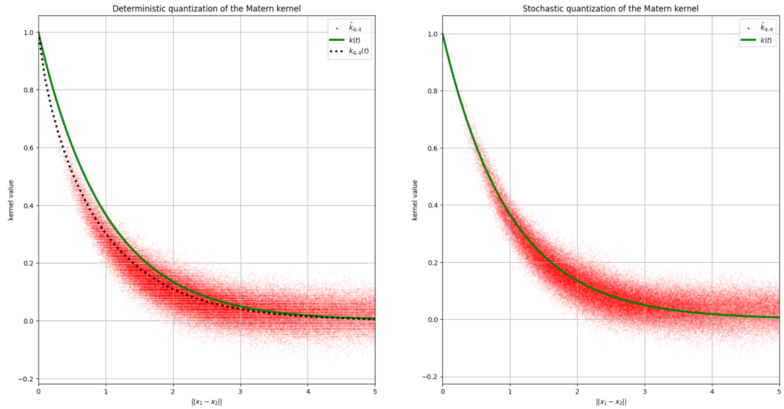
Figure 1.2: Comparison of different approximations of the Matern Kernel for M = 500 , \rho = 1 , \nu = 1/2 on the CASP dataset
