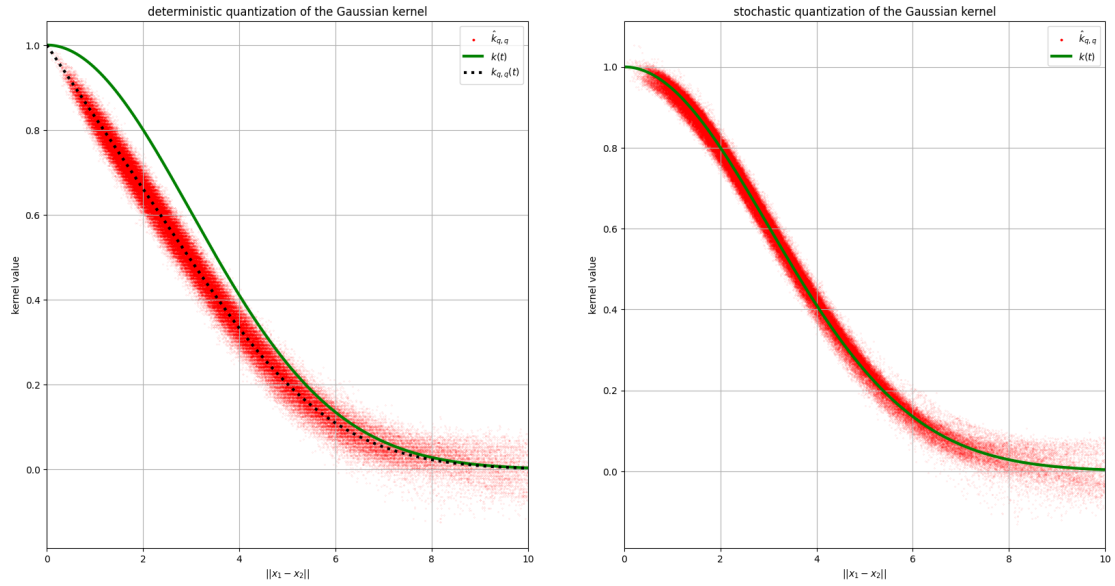
Figure 1.1: Comparison of different approximations of the Gaussian Kernel for M = 500 , \sigma = median-heuristic on the CASP dataset
