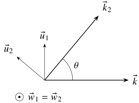
Figure 5: Polarization basis. The vectors \vec{u}_1, \vec{u}_2 lie in the scattering plane, while \vec{w}_1 = \vec{w}_2 points out of it.
