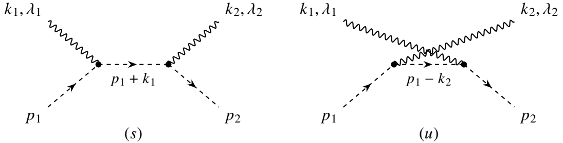
Figure 3: Virtual scalar exchange: s channel (left), u channel (right).
