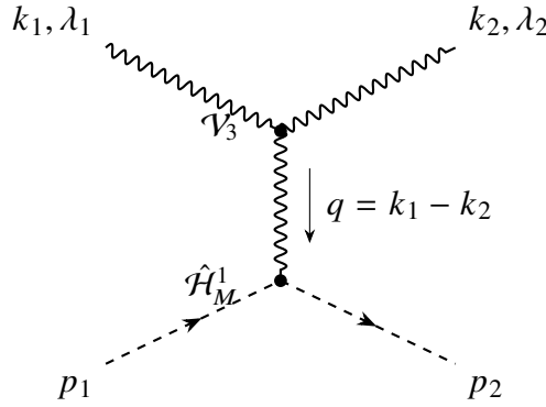
Figure 4: t -channel.
