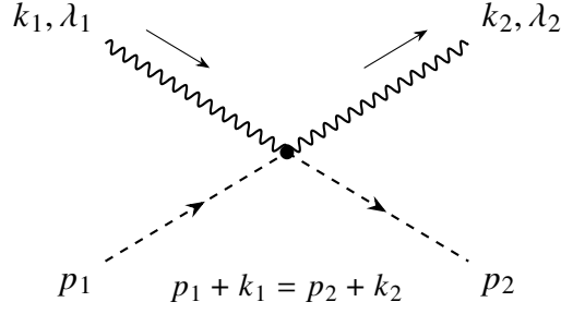
Figure 2: Seagull channel from \hat{\mathcal{H}}_M^2 .
