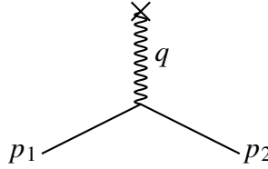
Figure 1: Straight line: scalar; wavy line: graviton
