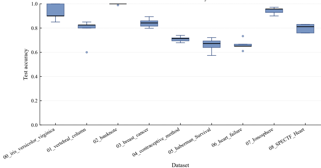
ModularNetwork: K-Fold accuracy distribution
