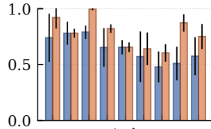
(c) Recall
