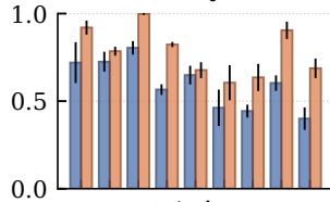
(a) Accuracy
