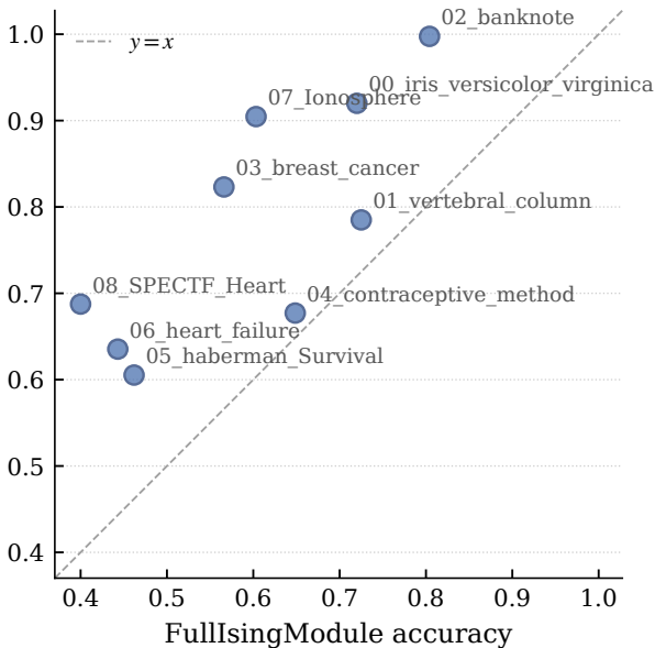
ModularNetwork accuracy
