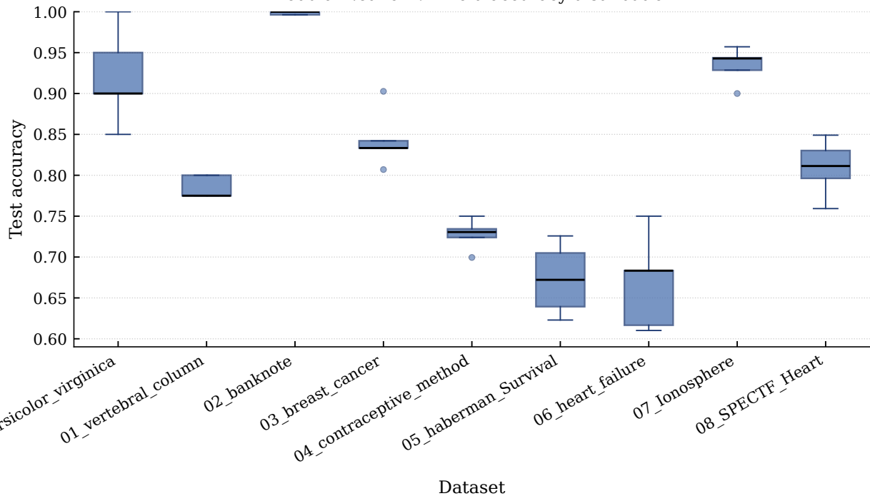
ModularNetwork: K-Fold accuracy distribution
