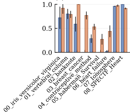
(c) Recall
