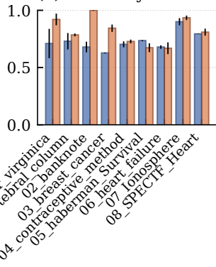
(a) Accuracy
