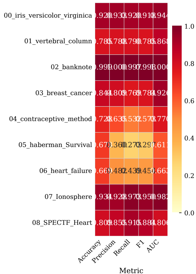
ModularNetwork
