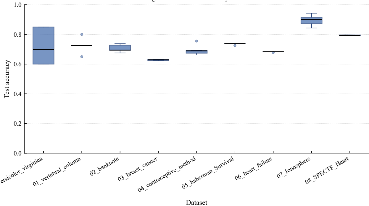
FullIsingModule: K-Fold accuracy distribution
