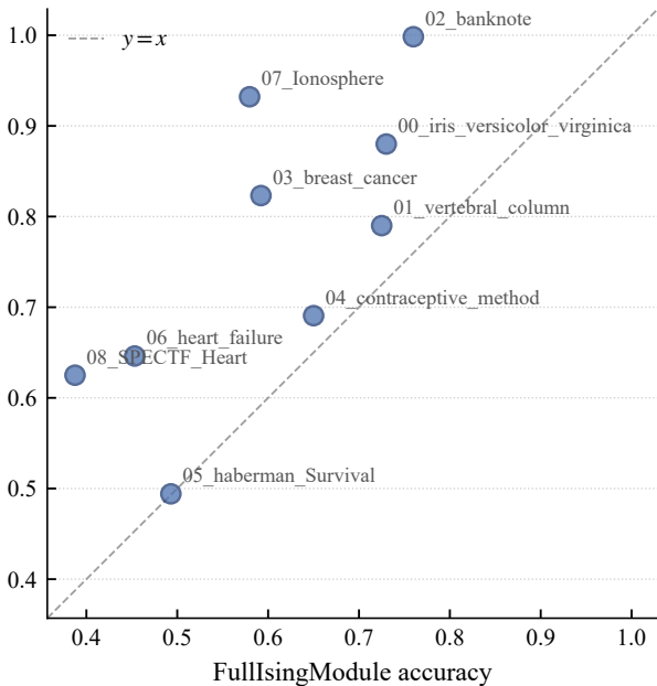
ModularNetwork accuracy
