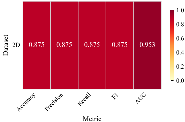
ModularNetwork
