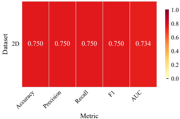
FullIsingModule
