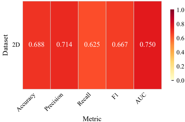
FullIsingModule
