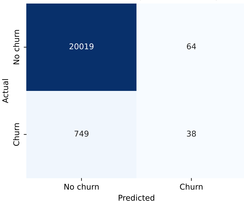
Confusion matrix (threshold = 0.5)
