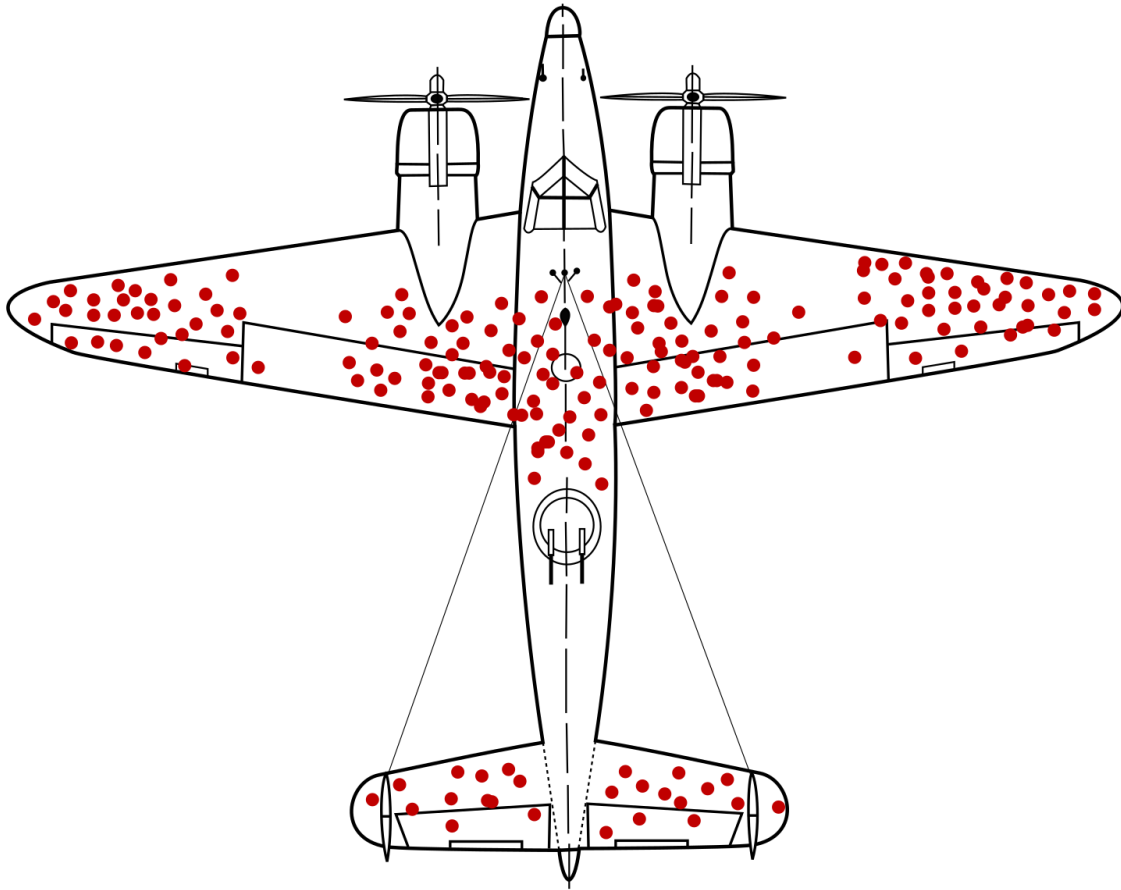
Figure 1.6: WWII bomber survivorship bias: hypothetical damage pattern on a returning aircraft. The areas without red dots are the ones that actually bring a plane down, since planes hit there never made it back. Source: Martin Grandjean, McGeddon, and the US Air Force, licensed under CC BY-SA 4.0.
