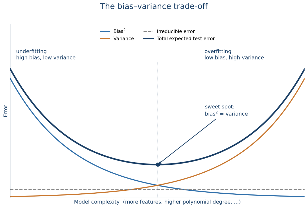
Figure 6.6: The bias–variance trade-off: as model complexity increases, bias 2 falls and variance rises. Total expected test error is their sum plus an irreducible noise floor, and its minimum falls exactly where the bias 2 and variance curves cross.
