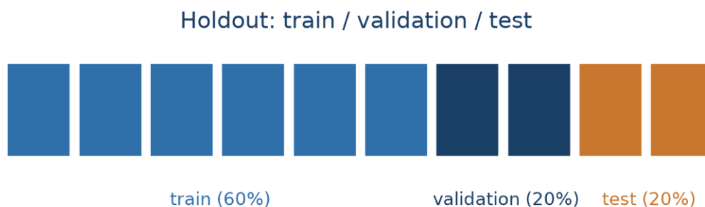
Figure 6.2: A three-way split: the validation set is used to compare models and pick hyperparameters, and only the test set is kept for the final measurement.
