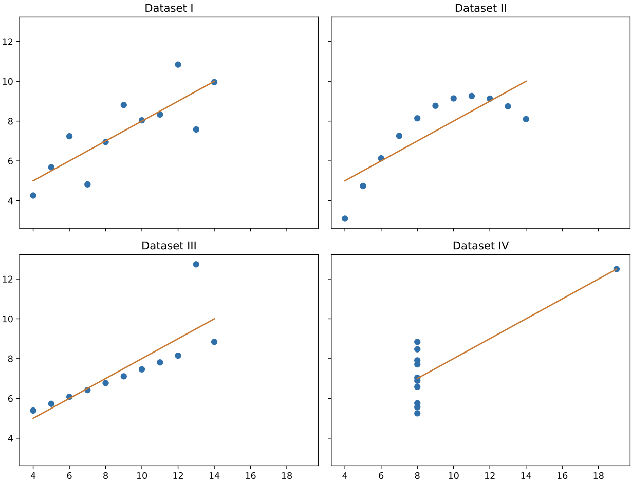
Anscombe's Quartet: identical statistics, very different data
