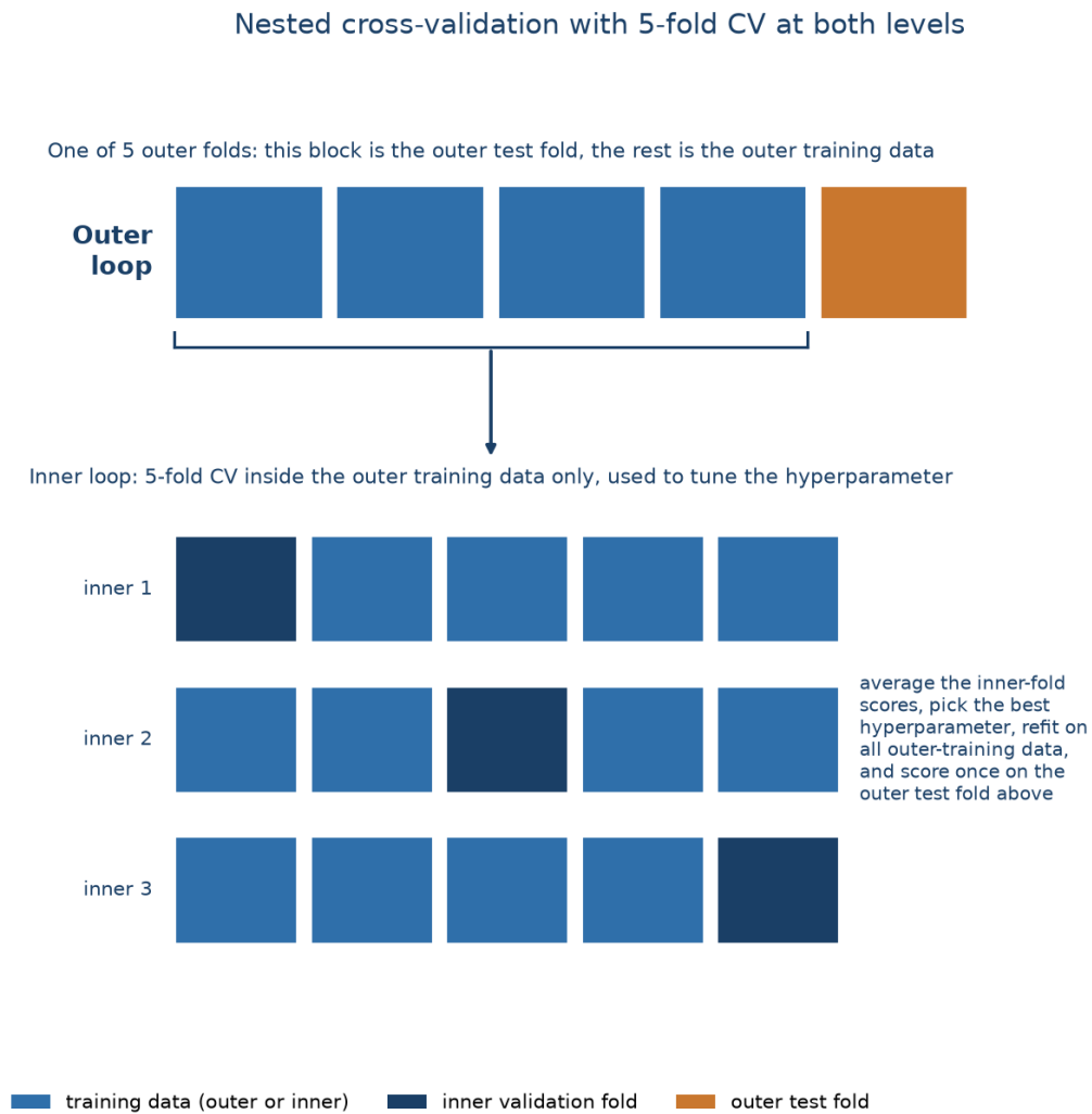
Figure 6.4: Nested cross-validation with 5-fold CV at both levels: one outer fold is shown on top, blue training data and an orange test fold; the arrow zooms into that training data below, where a second, inner 5-fold CV tunes the hyperparameter before the model is scored once on the outer test fold. The same logic applies for any choice of K .
