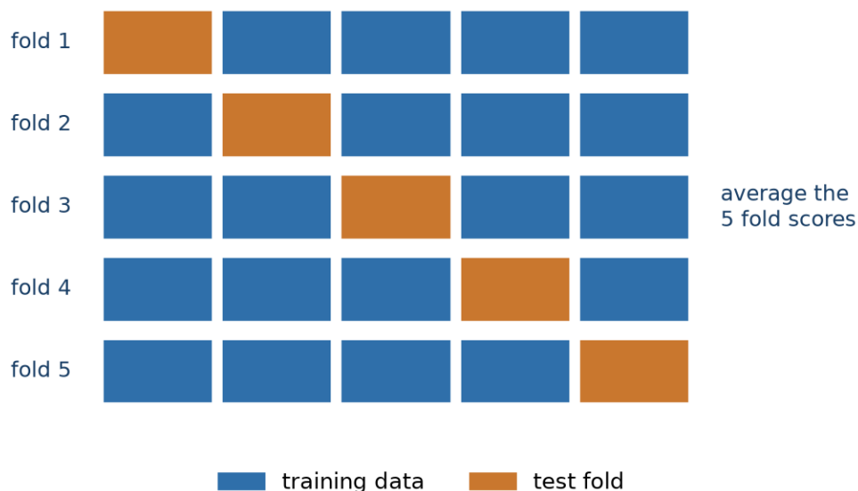
Figure 6.3: K-fold cross-validation: the data is cut into K folds, and each one takes a turn as the test set while the rest train the model.
