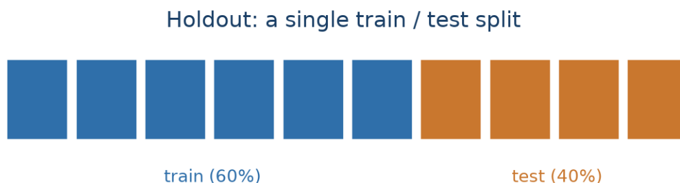
Figure 6.1: A single holdout split: most of the data trains the model, the rest is held back to test it.
