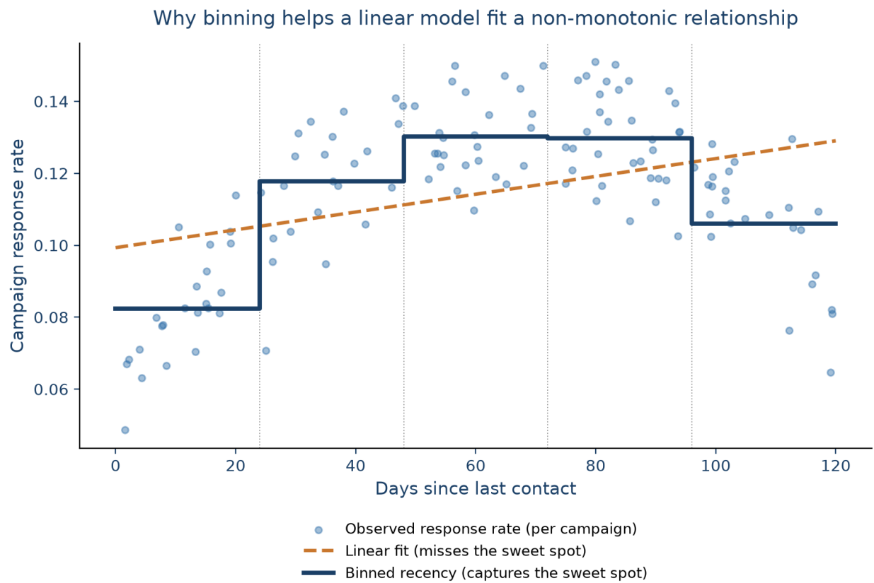
Figure 5.1: Why binning helps a linear model fit a non-monotonic relationship: a straight line (orange) averages away the rise-and-fall pattern, while a binned step function (navy) tracks it closely.
