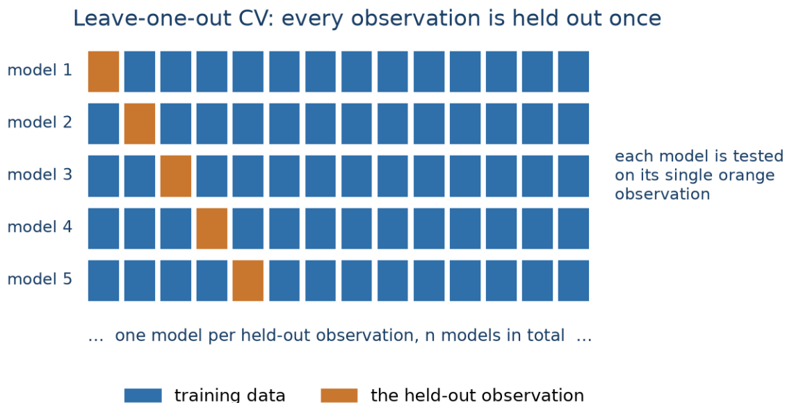
Figure 6.5: Leave-one-out cross-validation: each model trains on every row but one and is tested on that single held-out observation, for n models in total.
