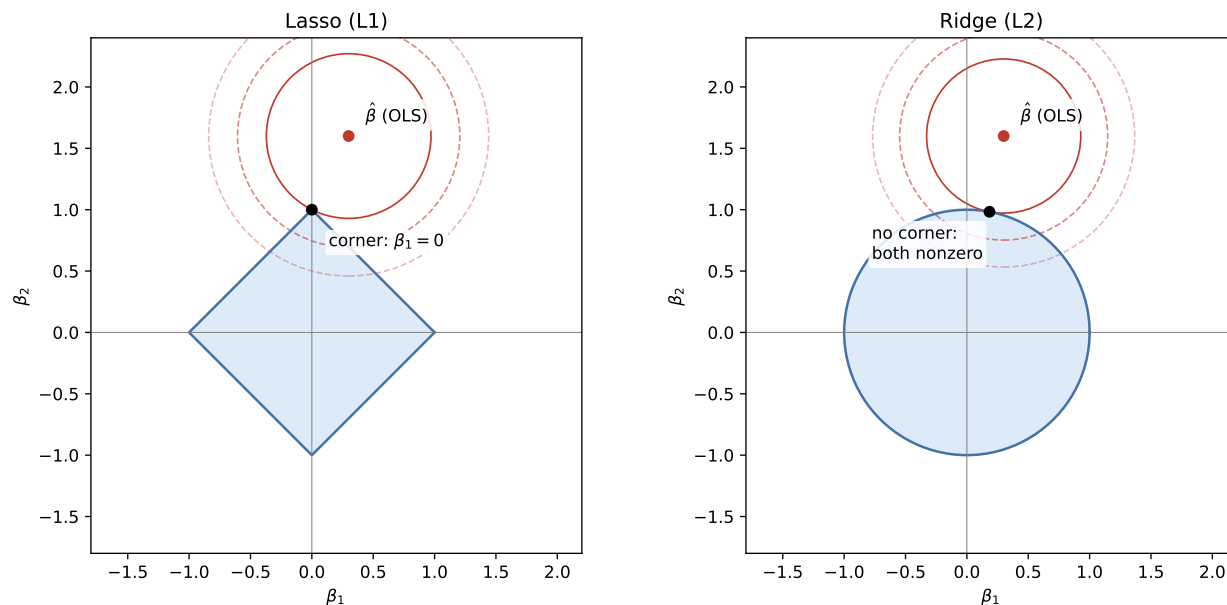
Figure 7.1: Why Lasso zeroes coefficients and Ridge doesn't: the diamond has corners on the axes, the circle has none.
