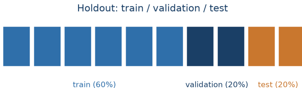
Figure 6.2: A three-way split: the validation set is used to compare models and pick hyperparameters, and only the test set is kept for the final measurement.
