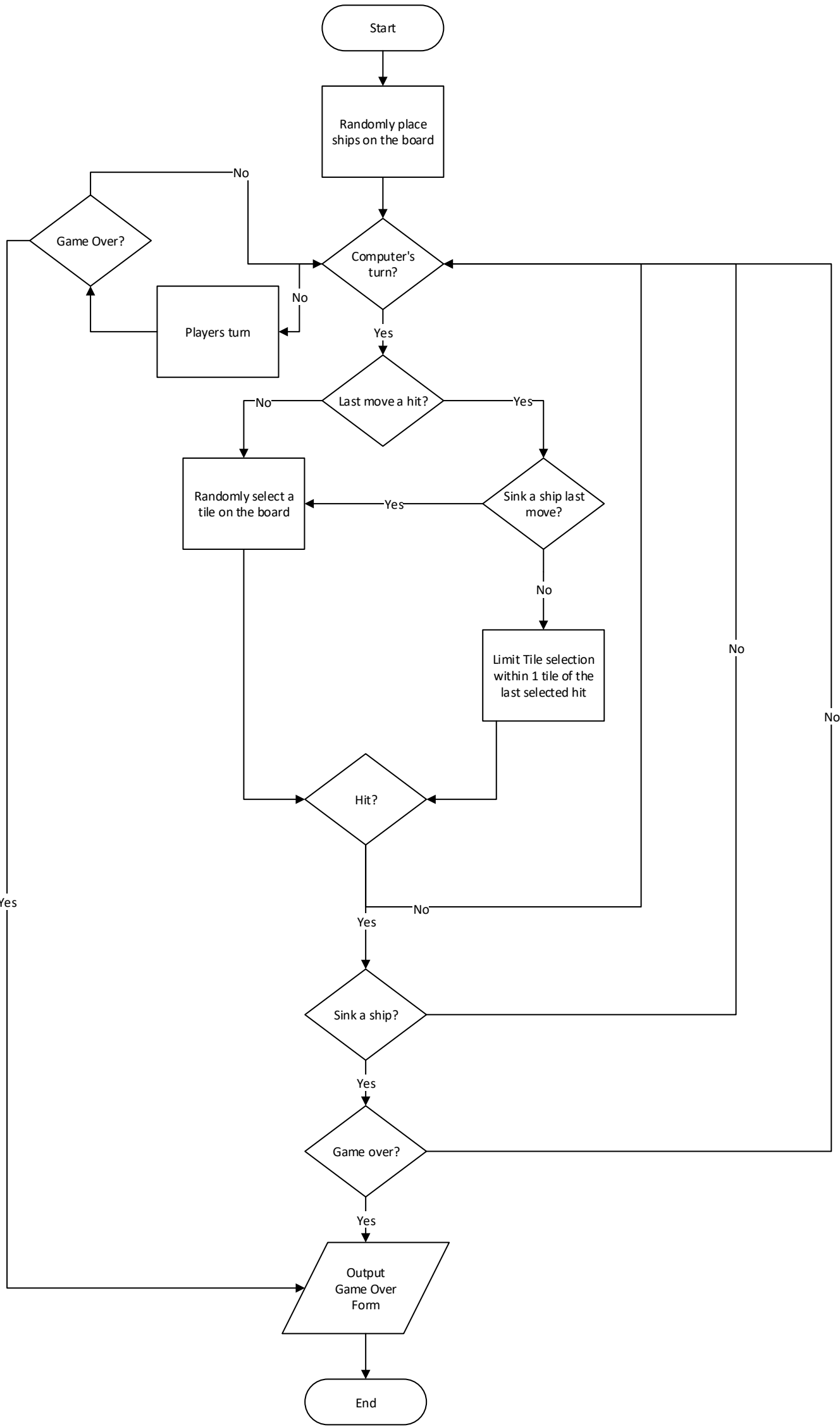
Computer Flowchart
