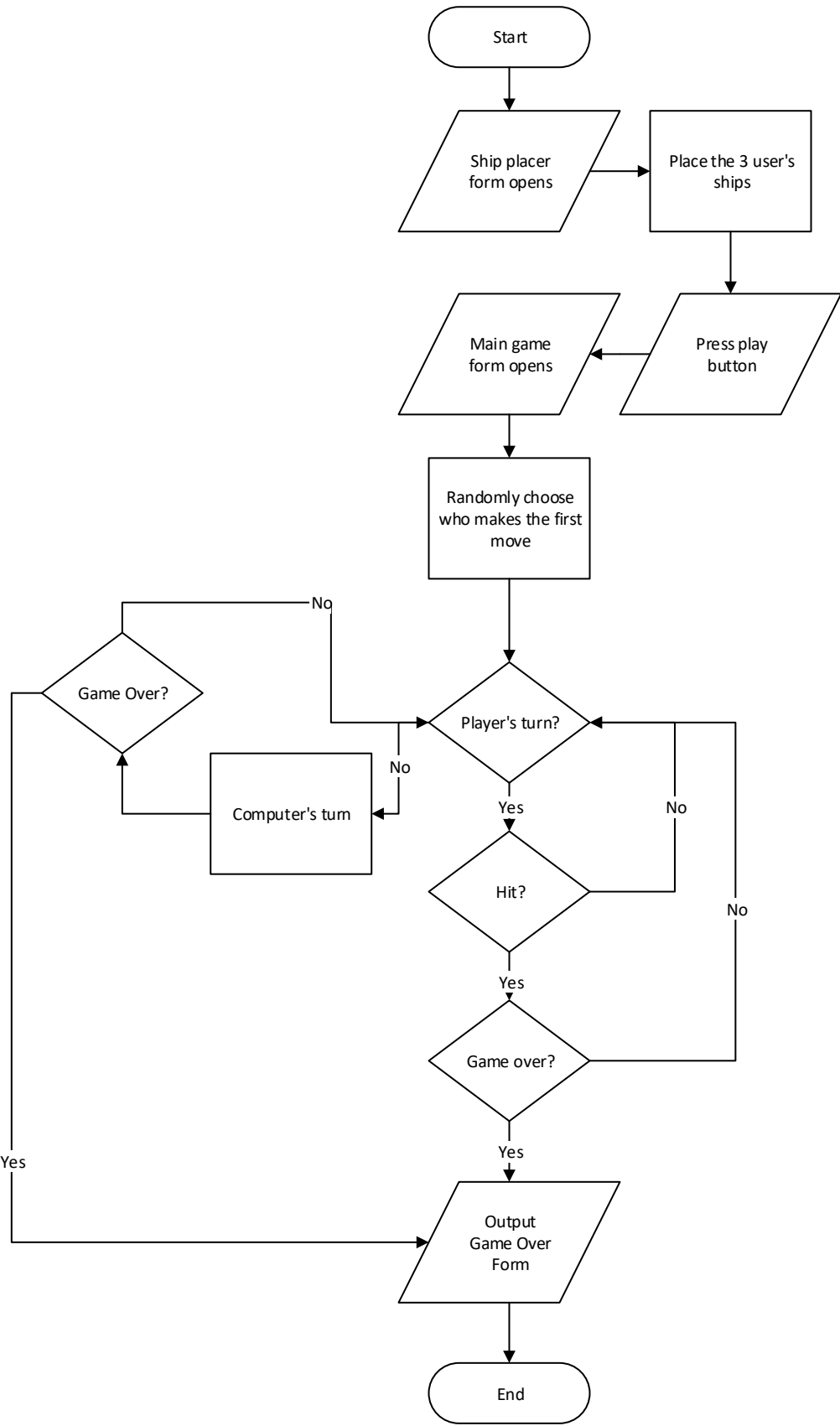
Player Flowchart
