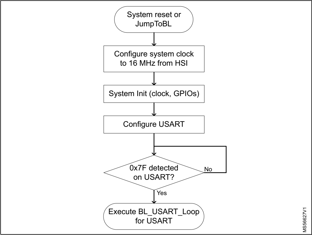
Figure 110. Bootloader V2.x selection for STM32WB05xx
