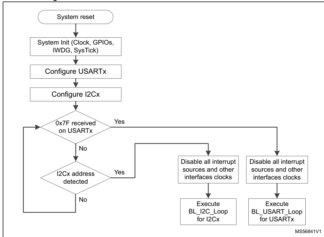
Figure 14. Bootloader V5.x selection for STM32C031xx devices
