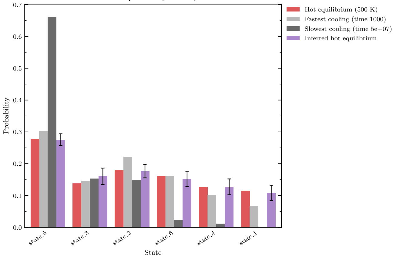
State-probability recovery
