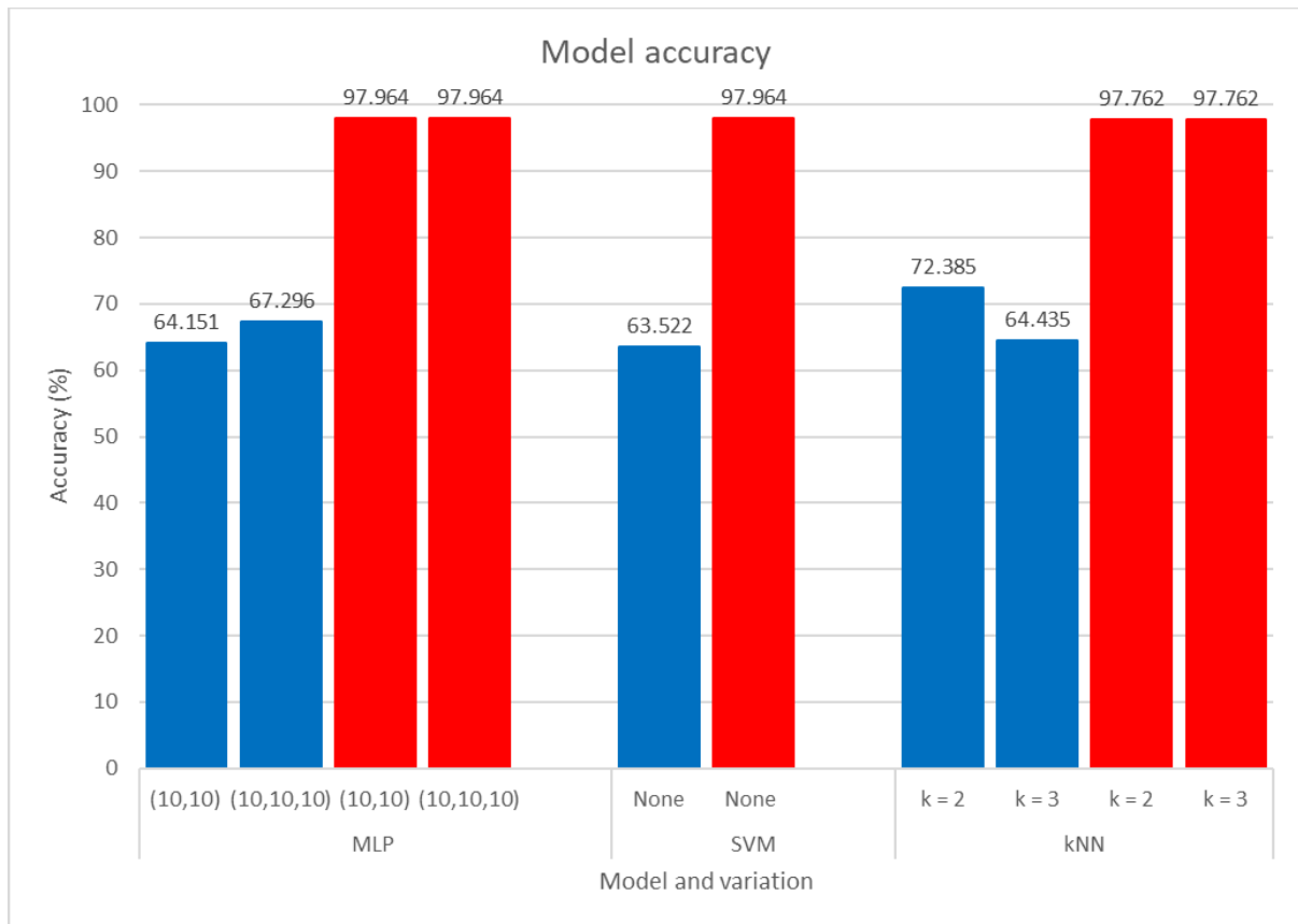
Figure 17: Graph of accuracy for each model
