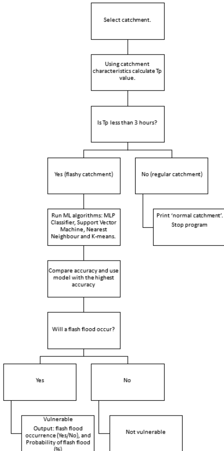
Figure 8: Flowchart displaying how SOPHIE measures vulnerability and expected outputs (See Appendix E-1)
