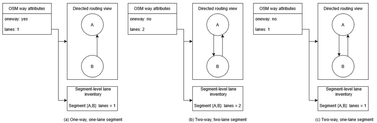
Figure 4.2 Relationship between the directed multigraph used for routing and the segment-level inventory used for physical lane supply. Directed arcs encode movement and accessibility, while segment records encode non-duplicated road-space supply.
