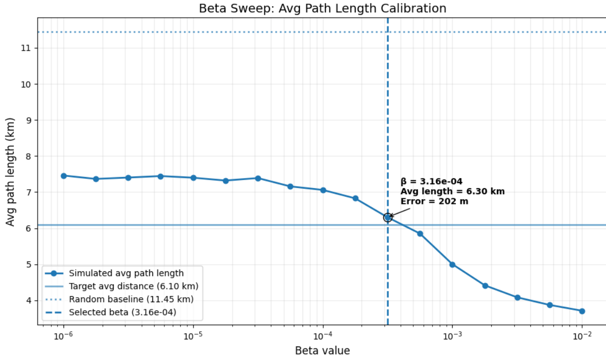
Figure 4.10 Calibration of the gravity-model distance-decay parameter \beta .
