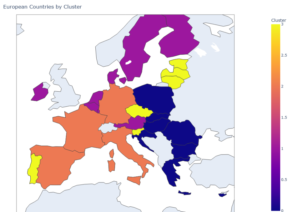
Figure 18: Country Clusters Map
