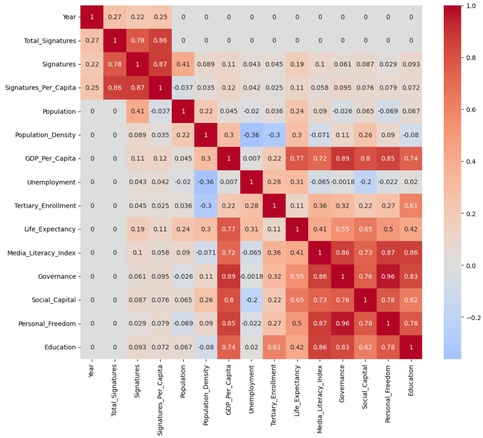
Figure 7: Spearman Heatmap for the Master Dataset
