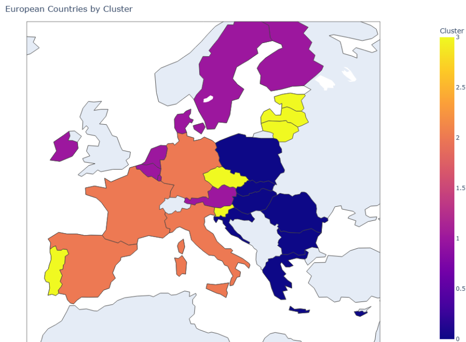
Figure 4: Country Clusters Map
