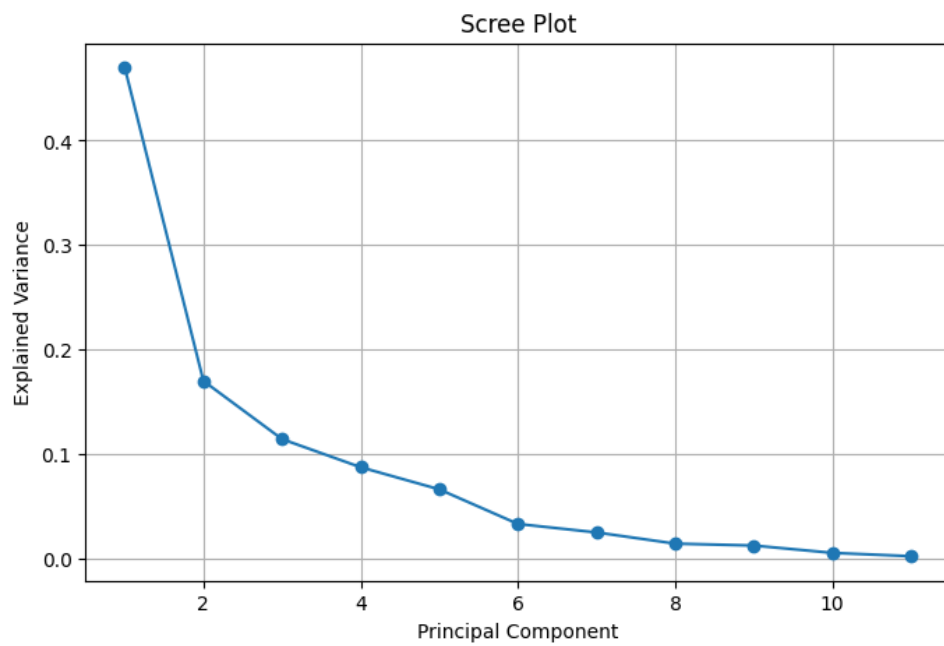
Figure 14: Scree Plot for PCA 02
