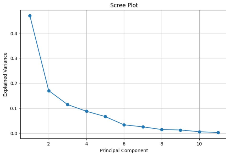
Figure 13: Scree Plot for PCA 01
