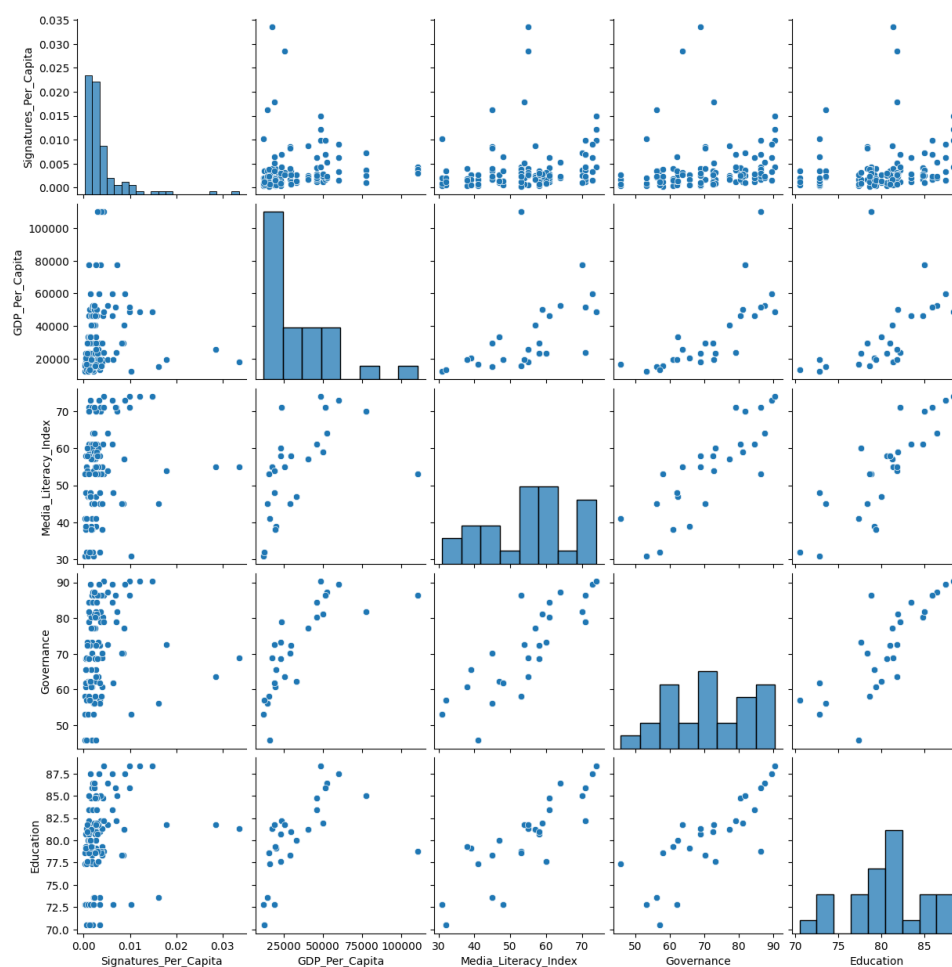
Figure 10: Pairplots for the Successful Dataset
