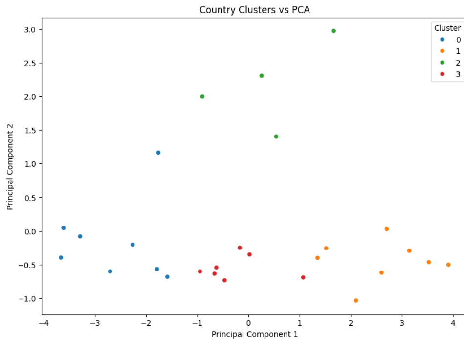
Figure 19: Clusters vs PCA Plot
