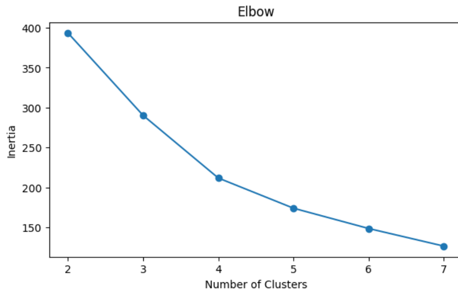
Figure 15: K Means Clustering Elbow
