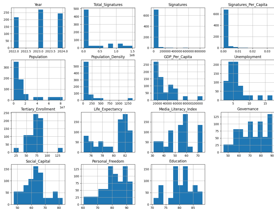
Figure 6: EDA Histograms
