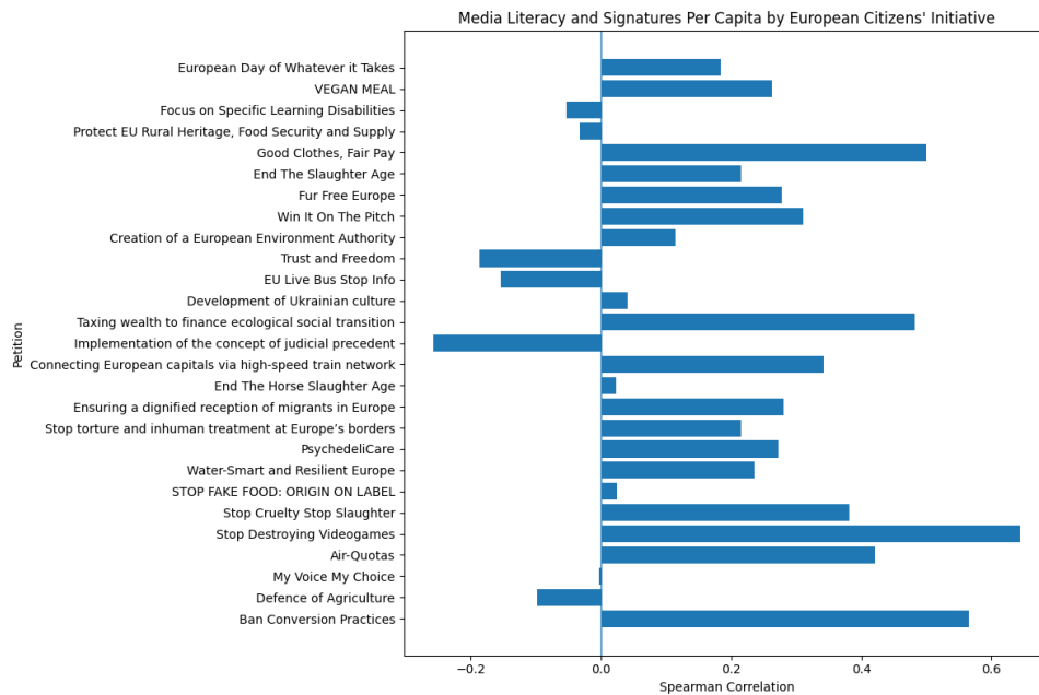
Figure 12: Correlations Signatures Per Capita vs Media Literacy grouped by Petition
