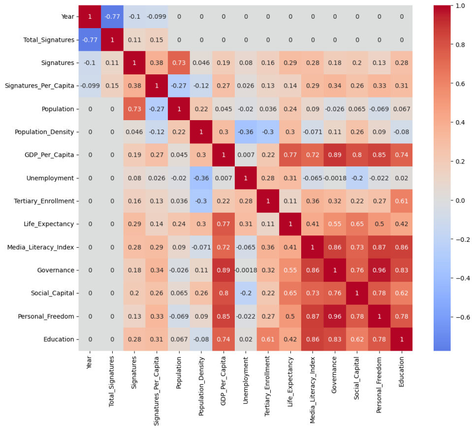
Figure 8: Spearman Heatmap for the Successful Dataset
