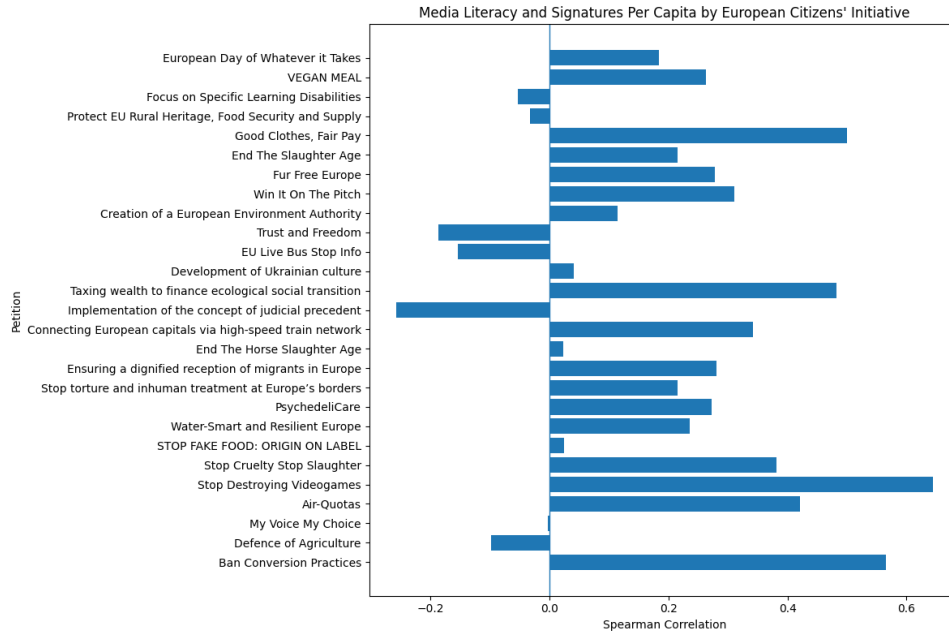
Figure 2: Correlations Signatures Per Capita vs Media Literacy grouped by Petition
