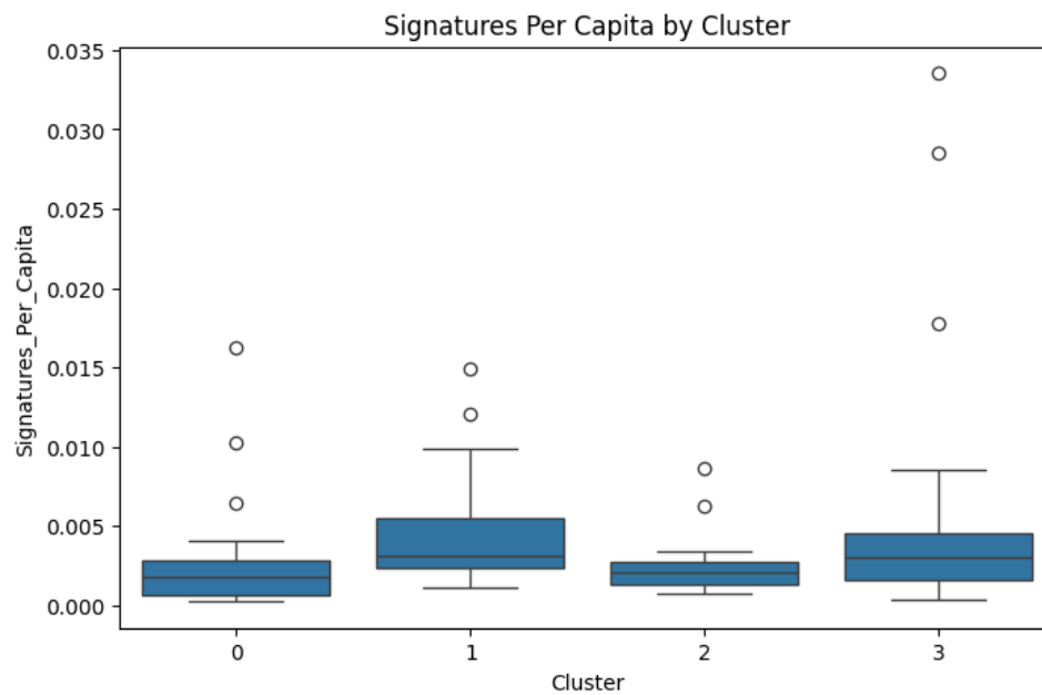
Figure 16: Signatures Per Capita by Cluster
