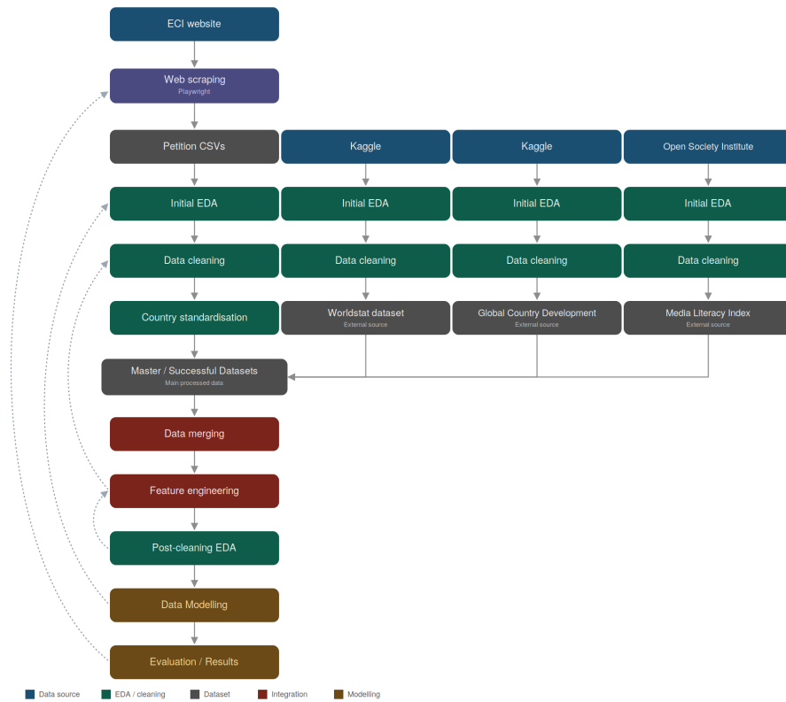
Figure 5: Project Workflow Chart
