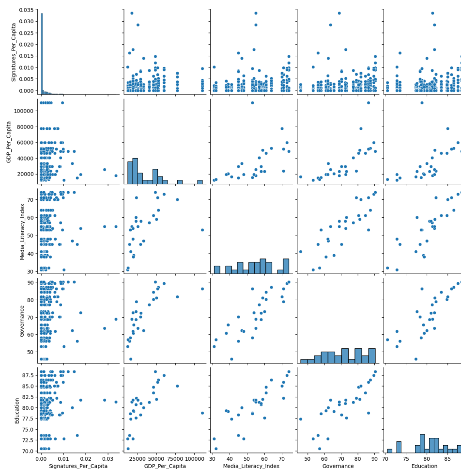
Figure 9: Pairplots for the Master Dataset
