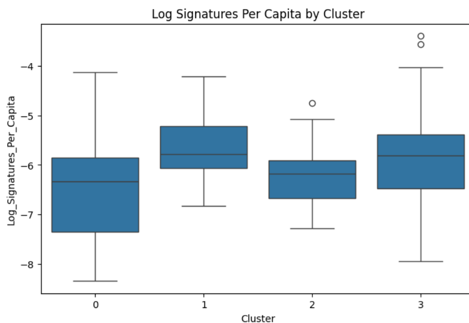
Figure 17: Log Signatures Per Capita by Cluster
