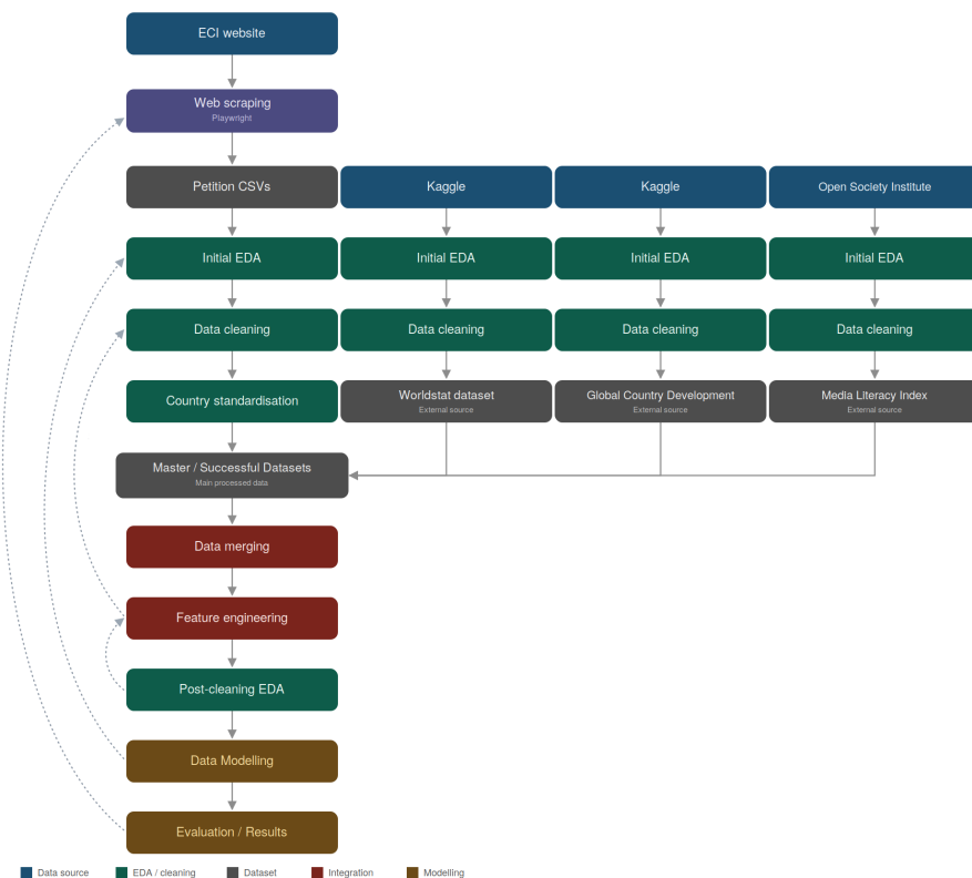
Figure 3: Project Workflow Chart
