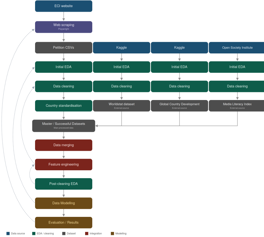
Figure 1: Project Workflow Chart
