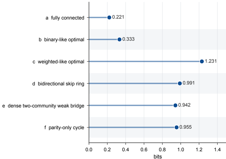
a Total effective information
