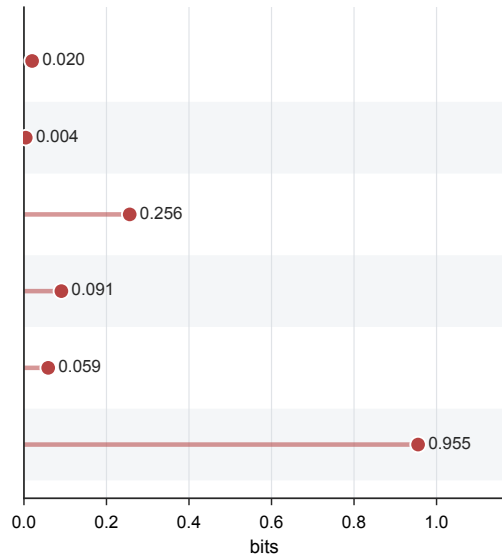
b Highest-order synergy, \Phi^{\text{EID}}
