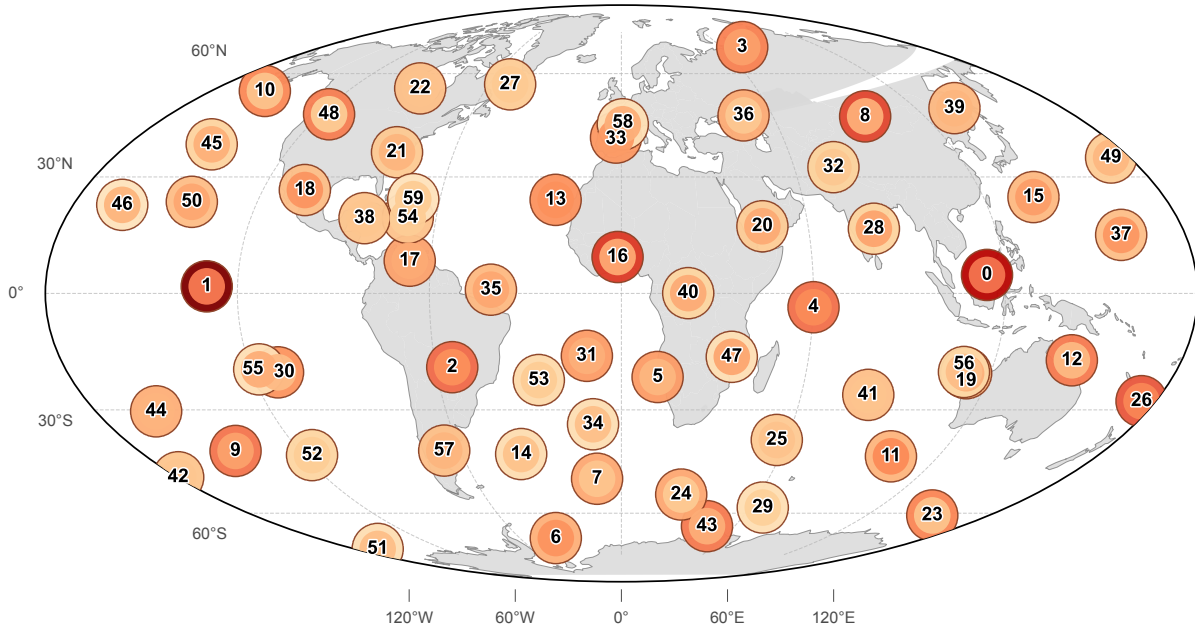
Runge 2015 method (PC-stable), new 1948-2026 data
