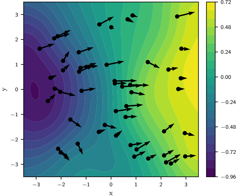
Posterior Mean (conditioned on \nabla f )
