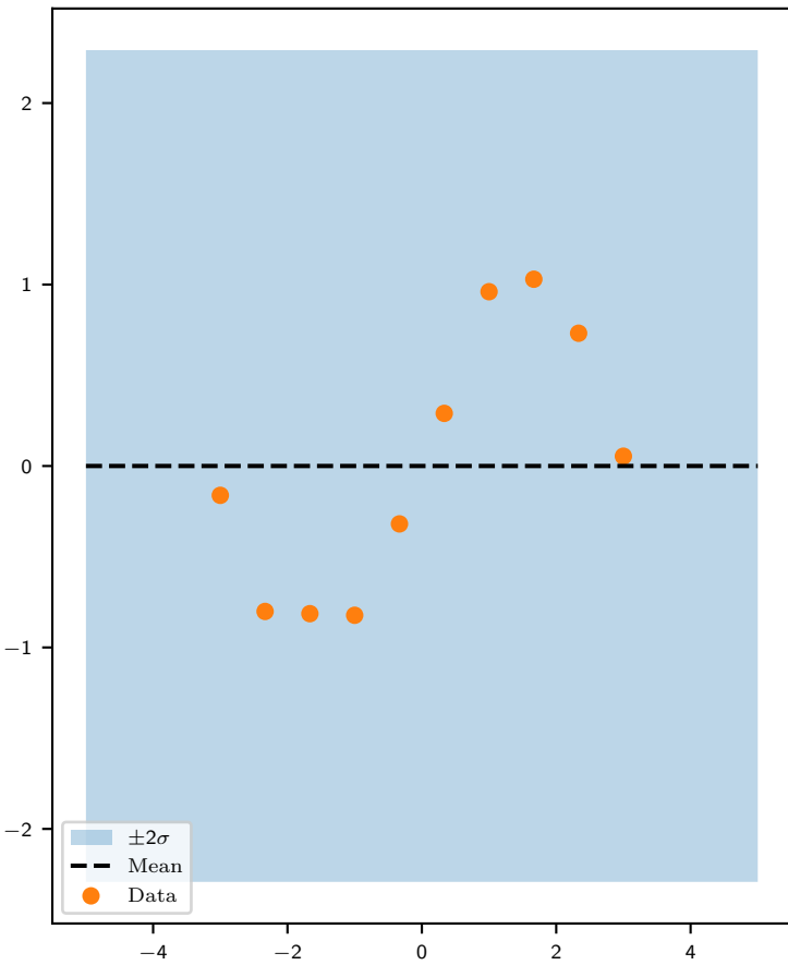
Prior GP (RBF)
