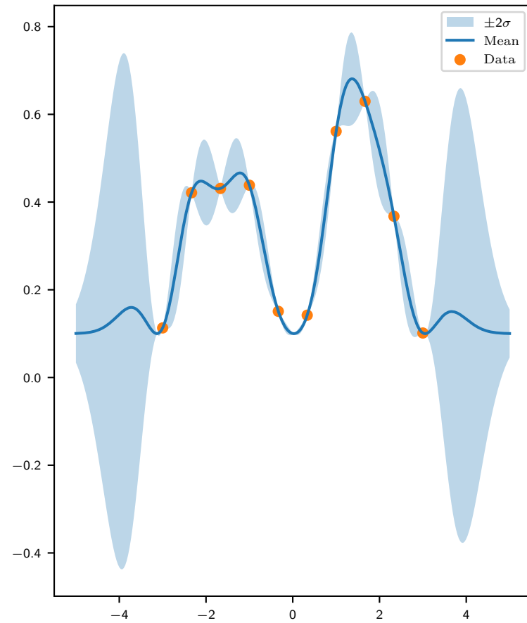
Linearised g Warp
