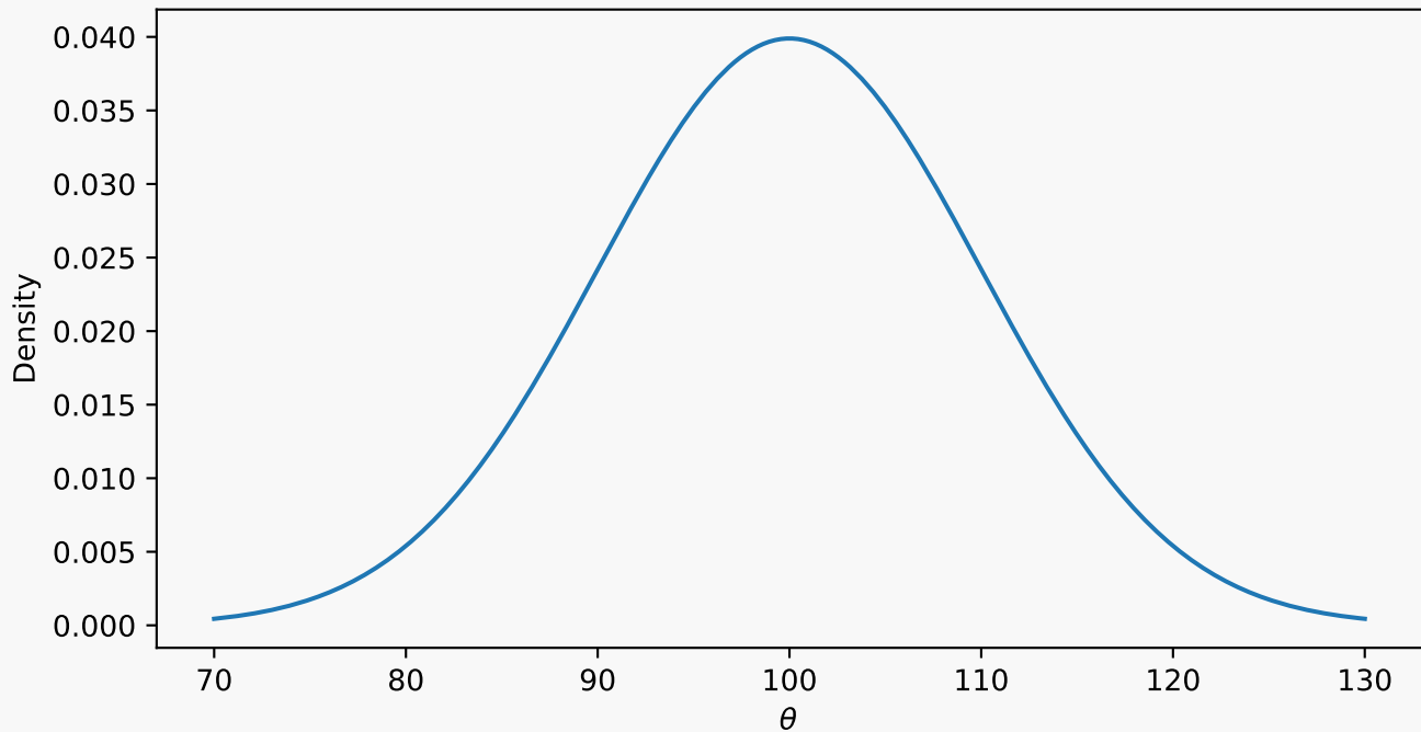
Normal PDF: mean = 100, sd = 10
