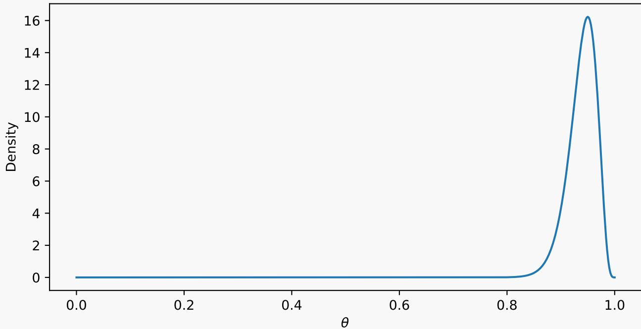
Beta PDF: \alpha = 77, \beta = 5
