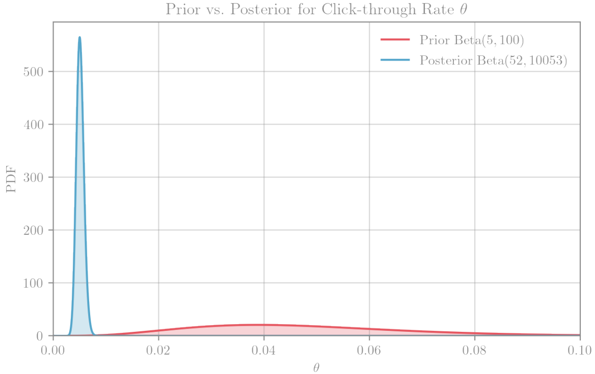
Figure 12.1: Beta prior and posterior for the Instagram click-through rate parameter \theta after observing X = 47 clicks out of n = 10,000 impressions. The posterior is sharply concentrated near \sim 0.5\%
