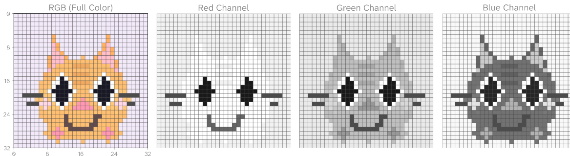
Figure 4.1: A 32 \times 32 image of a cat, broken into its three colour channels (red, green, blue). Each pixel has three values (one per channel), making the image a high-dimensional observation.
