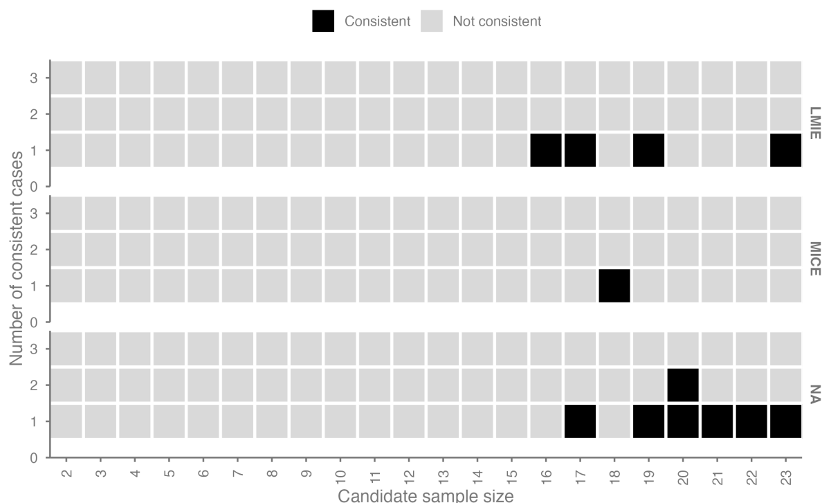
Figure 3: GRIMMER consistency across candidate sample sizes. Black tiles indicate PHQ-9 mean-SD pairs that are GRIMMER-consistent; light grey tiles indicate inconsistent pairs. No group has any candidate sample size below n = 23 for which all three timepoints are simultaneously consistent.
