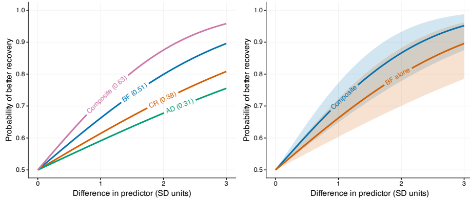
Figure 3: POSCs for a composite of several predictors. Left: curves for three single prognostic measures and for their optimally weighted composite, from the illustrative correlation matrix of Section 5: baseline function (BF, correlation 0.51 with recovery), clinician rating (CR, 0.38), treatment adherence (AD, 0.31), and the composite (unadjusted multiple correlation 0.63). Right: the composite and the best single measure (BF) estimated from n = 100 patients, with 95% confidence bands (approximate for the composite). Labels sit on the curves.
