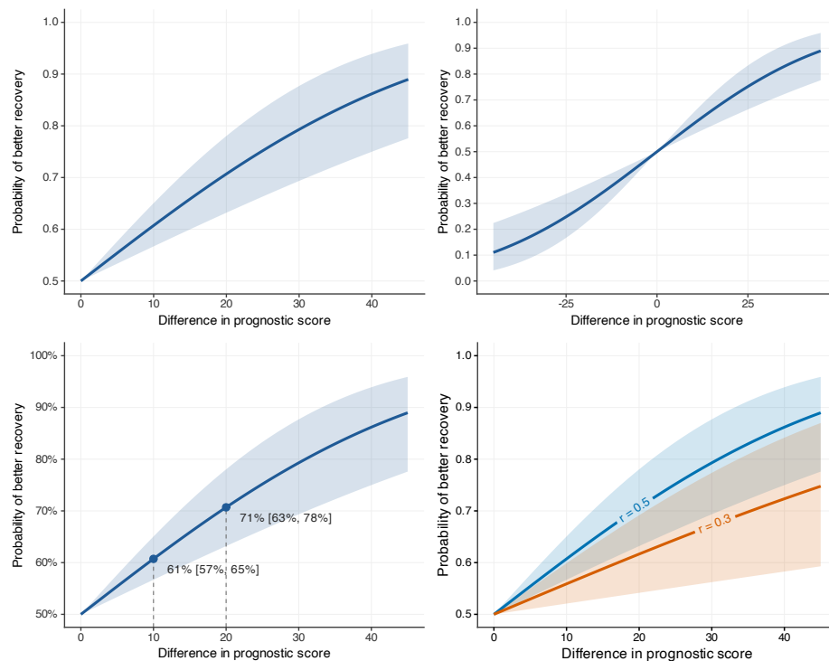
Figure 6: The plot method for a curve from posc_uni(r = 0.5, n = 100, sd_x = 15) . Top left: the default, the curve over positive differences with its 95% confidence band. Top right: full = TRUE , the full sigmoid. Bottom left: mark = c(10, 20) , mark_ci = TRUE and percent = TRUE , which label chosen differences with their probabilities and confidence intervals on a percentage axis. Bottom right: a comparison of two curves from posc_comp() , labelled along the curves.
