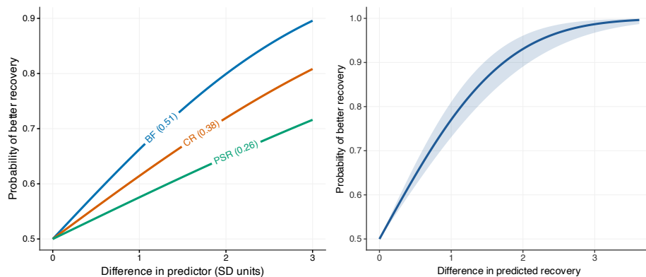
Figure 8: POSCs for three prognostic measures and for a linear model. Left: normal-theory curves for three prognostic measures with illustrative correlations with recovery: a baseline functional assessment (BF, 0.51), a clinician’s global rating (CR, 0.38) and a patient self-rating (PSR, 0.26). Right: the curve for the fitted values of a linear model with two predictors fitted to 200 simulated patients, with its 95% confidence band; the difference on the horizontal axis is in units of predicted recovery.
