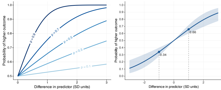
Figure 2: Normal-theory POSCs. Left: curves for population correlations \rho from 0.1 to 0.9 over differences of 0 to 3 standard deviations of the predictor, each labelled along its path. Right: the full curve for \rho = 0.5 estimated from n = 100 , over negative and positive differences, with its 95% confidence band. The curve passes through 0.5 at a difference of zero and is point-symmetric about that point, so the two halves carry the same information. Marked points show the probabilities at differences of one standard deviation in each direction.
