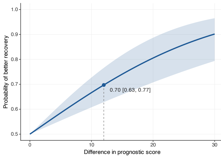
Figure 7: POSC for a prognostic score with r = 0.52 , n = 100 and s_X = 10 . The shaded region is the 95% confidence band. The marked point is the 12-point difference between the two patients, with its probability and confidence interval.
