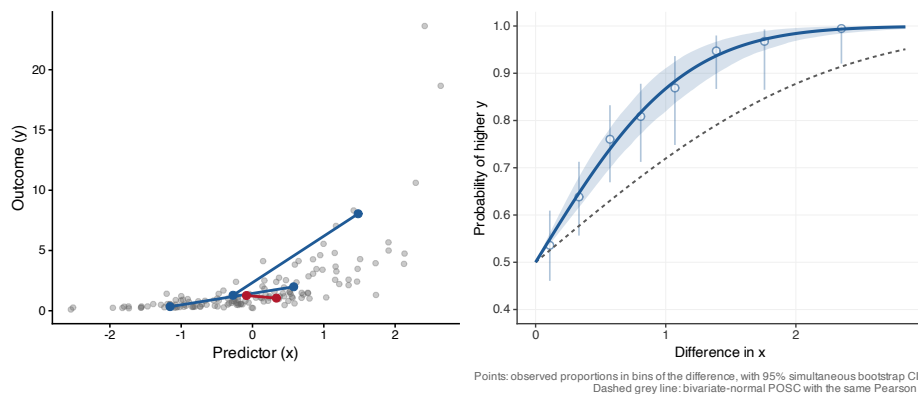
Figure 4: Construction of an empirical POSC. Left: 150 simulated observations with a skewed outcome ( y = \exp(0.8x + \epsilon) ); three of the 11,175 pairs are drawn as segments, blue if concordant (the observation higher on x is also higher on y ) and red if discordant. Right: the empirical POSC (solid line) with its 95% bootstrap band, the observed proportion of concordant pairs in eight bins of |\Delta| with 95% simultaneous intervals (points and whiskers), and the normal-theory curve for the same Pearson correlation (dashed).
