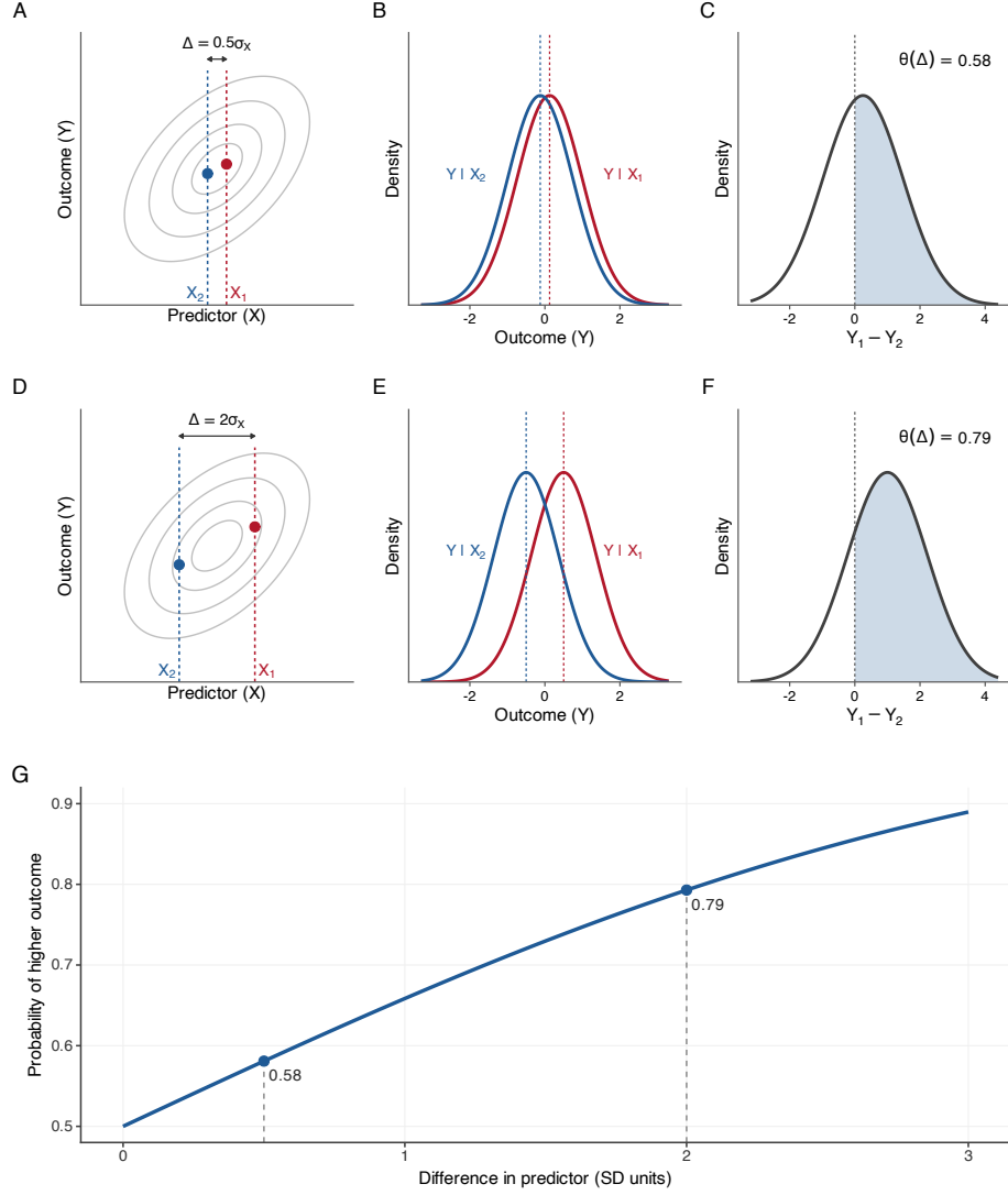
Figure 1: From the bivariate normal distribution to the POSC, for \rho = 0.5 and a predictor in standard deviation units. Panels A to C concern two people whose predictor scores differ by a small amount, \Delta = X_1 - X_2 = 0.5\sigma_X ; panels D to F concern two people who differ by a large amount, \Delta = 2\sigma_X . A, D: contours of the joint distribution of X and Y ; the dashed lines mark the predictor scores X_2 (blue) and X_1 (red) of the two people, and the points mark the conditional means of the outcome. B, E: the conditional distributions of the outcome, Y | X_2 (blue) and Y | X_1 (red), which are normal with the same variance and with means separated in proportion to \rho\Delta . C, F: the distribution of the difference Y_1 - Y_2 given \Delta , Equation 8; the shaded area above zero is \theta(\Delta) = P(Y_1 > Y_2 | \Delta) , Equation 9, which increases from 0.58 to 0.79 as \Delta increases. G: the POSC for \rho = 0.5 with the two differences marked; the shaded areas in C and F are the heights of the curve at those differences.
