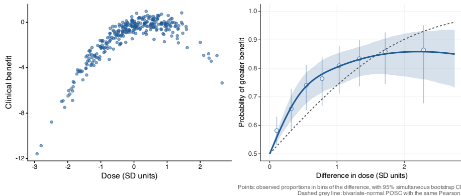
Figure 5: An inverted-U dose-response relationship. Left: simulated clinical benefit as an inverted-U function of dose with its optimum 0.5 standard deviations above the mean dose ( n = 300 ). Right: the empirical POSC (solid line) with its 95% bootstrap band and binned proportions, and the normal-theory curve for the same Pearson correlation (dashed); the normal-theory curve rises toward 1 while the empirical curve plateaus near \Phi(0.5\sqrt{2}) = 0.76 .
