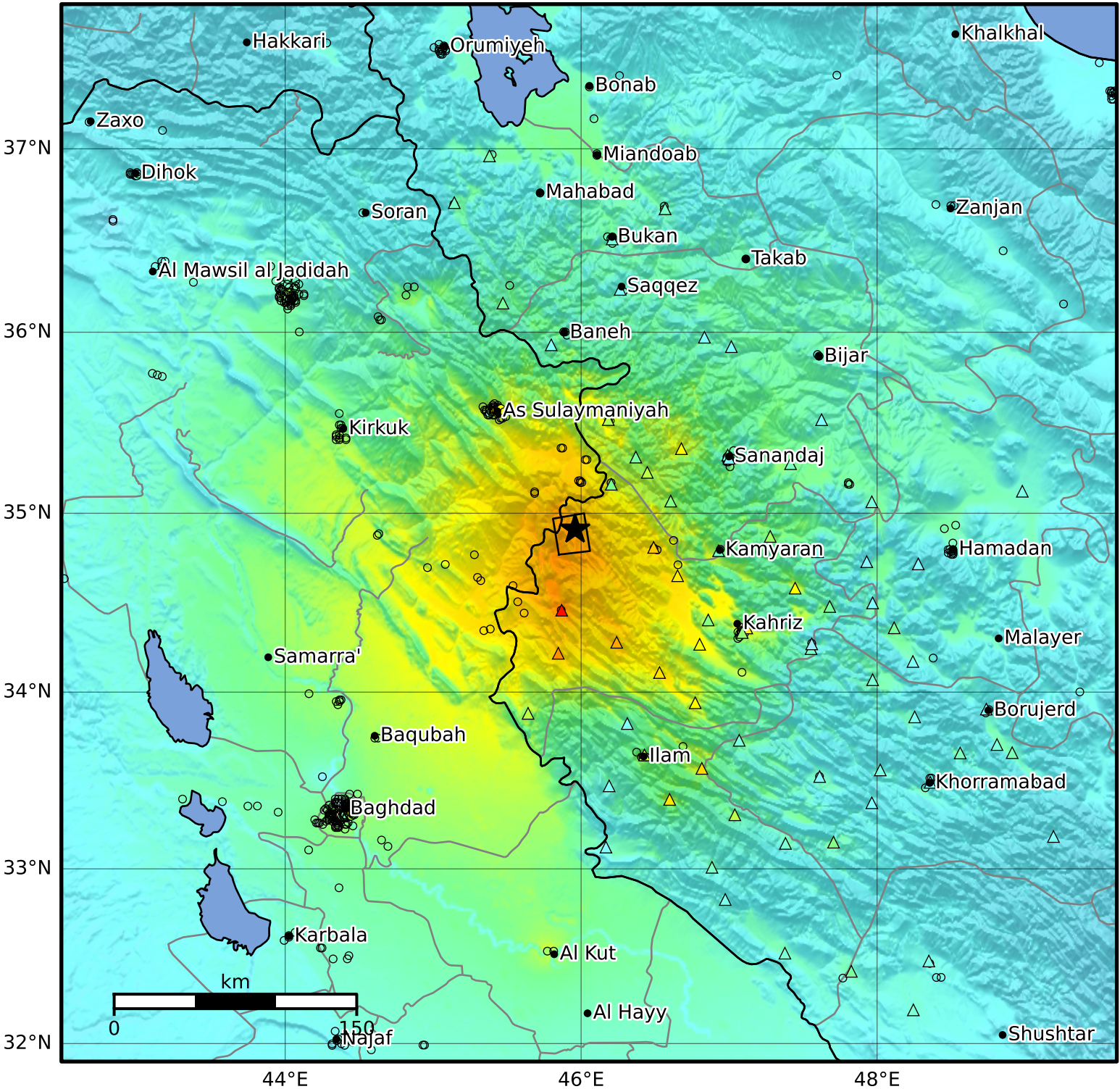
Macroseismic Intensity Map USGS ShakeMap: 29 km S of ?alabja, Iraq Nov 12, 2017 18:18:17 UTC M7.3 N34.91 E45.96 Depth: 19.0km ID:us2000bmcg
