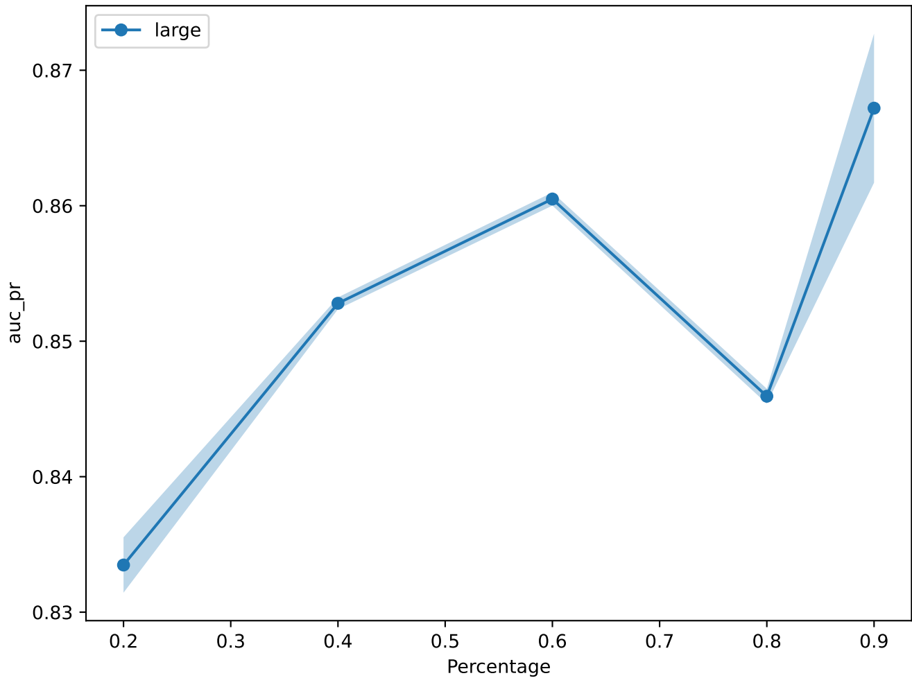
TUAB auc_pr vs Percentage
