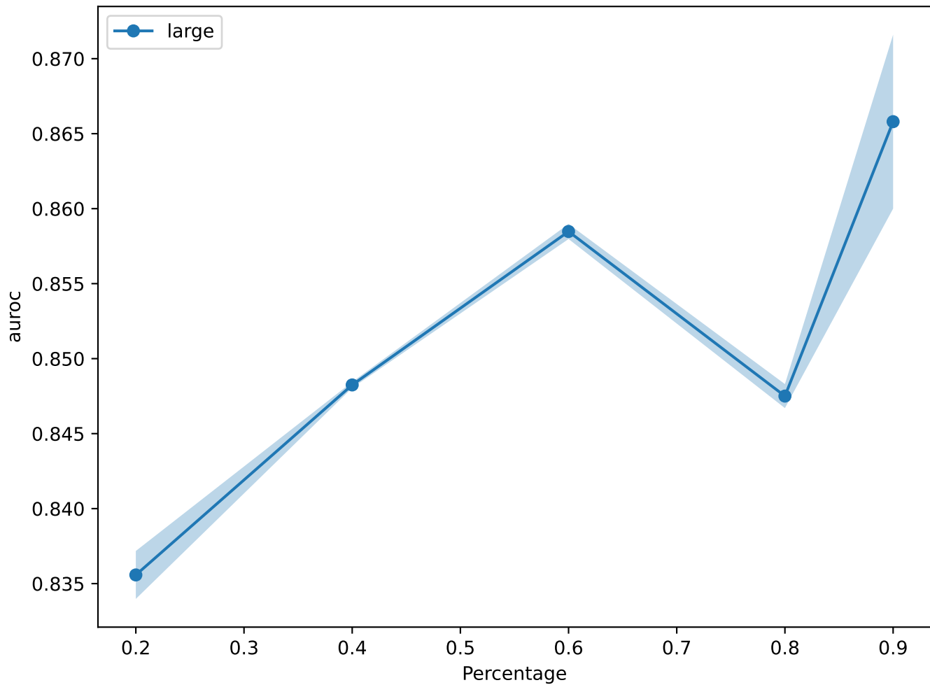
TUAB auroc vs Percentage
