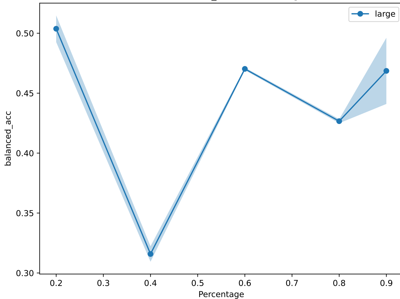
TUAB balanced_acc vs Percentage
