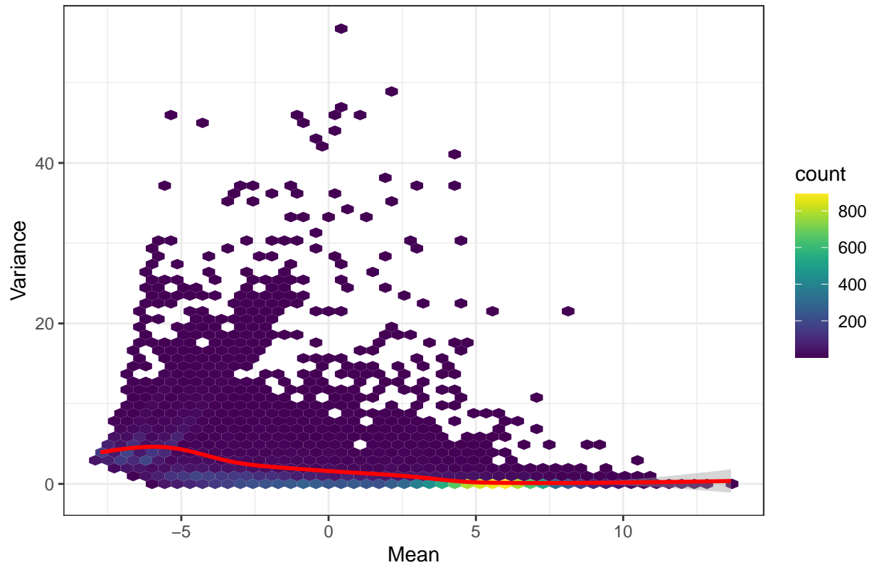
Mean-Variance Relationship
