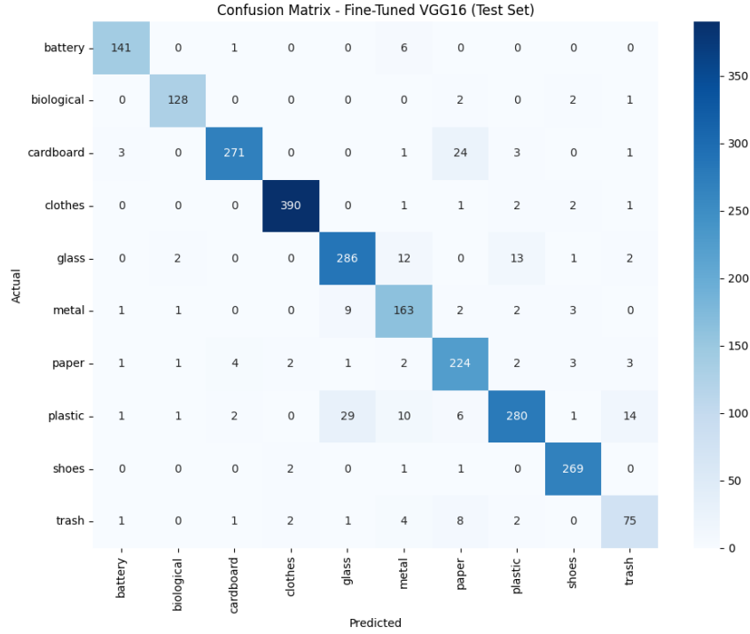
Figure 3: Confusion matrix for the fine-tuned VGG16 on the held-out test set.
